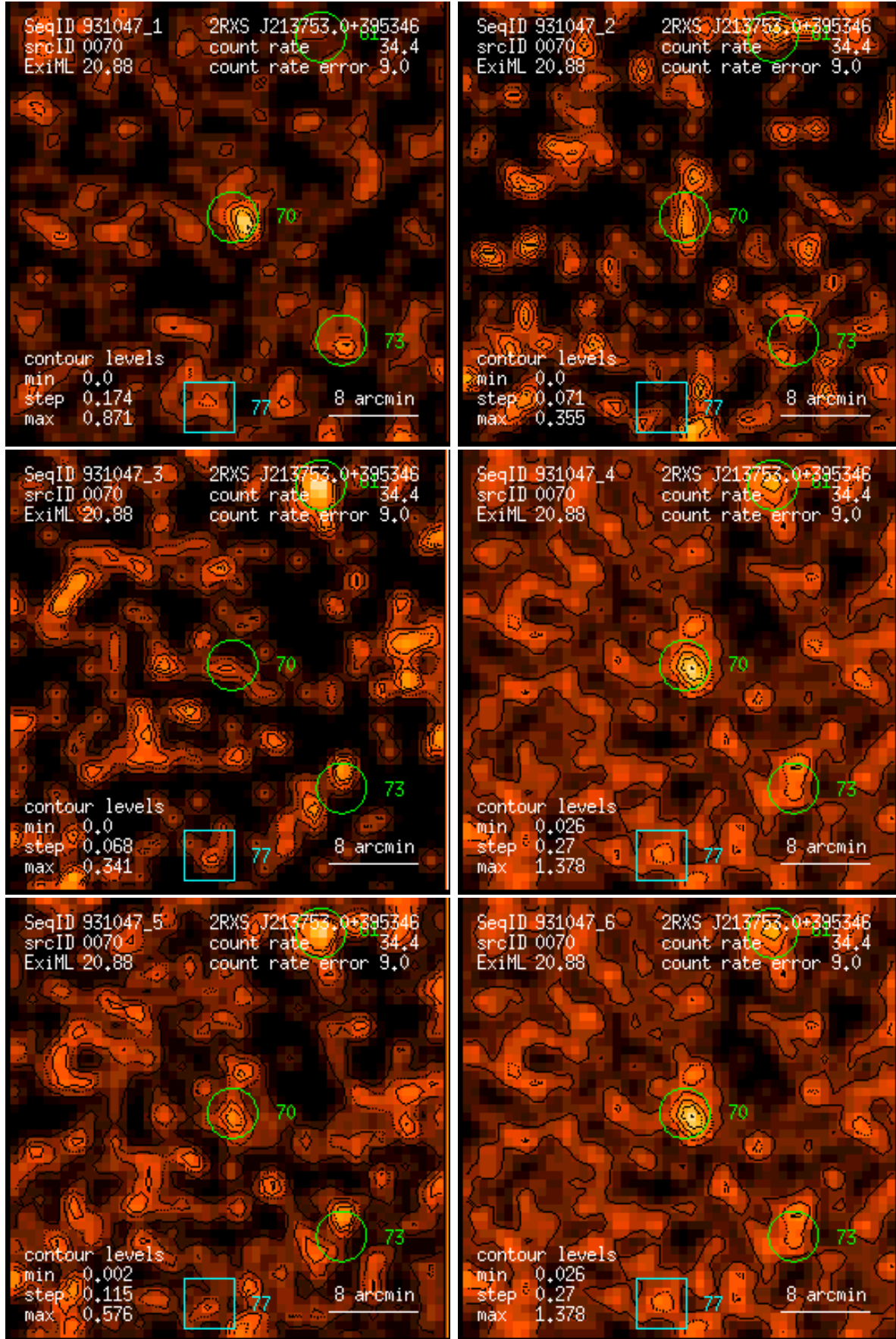
Figure 70: RASS 931047: detection 0070: band rate images, Gaussian filter: (1) PSPC channels 11 – 41, (2) 52 – 90, (3) 91 – 201, (4) 11 – 235, (5) 52 – 201, (6) 11 – 201. Broad band rates in counts/ks. Band rate contour levels in counts/ks/arcmin 2 .
