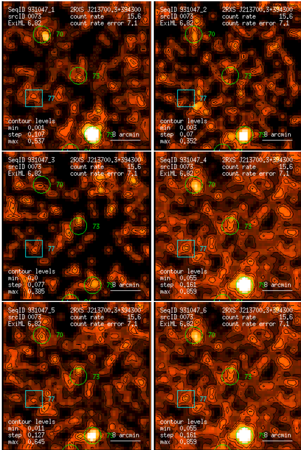
Figure 73: RASS 931047: detection 0073: band rate images, Gaussian filter: (1) PSPC channels 11 – 41, (2) 52 – 90, (3) 91 – 201, (4) 11 – 235, (5) 52 – 201, (6) 11 – 201. Broad band rates in counts/ks. Band rate contour levels in counts/ks/arcmin 2 .
