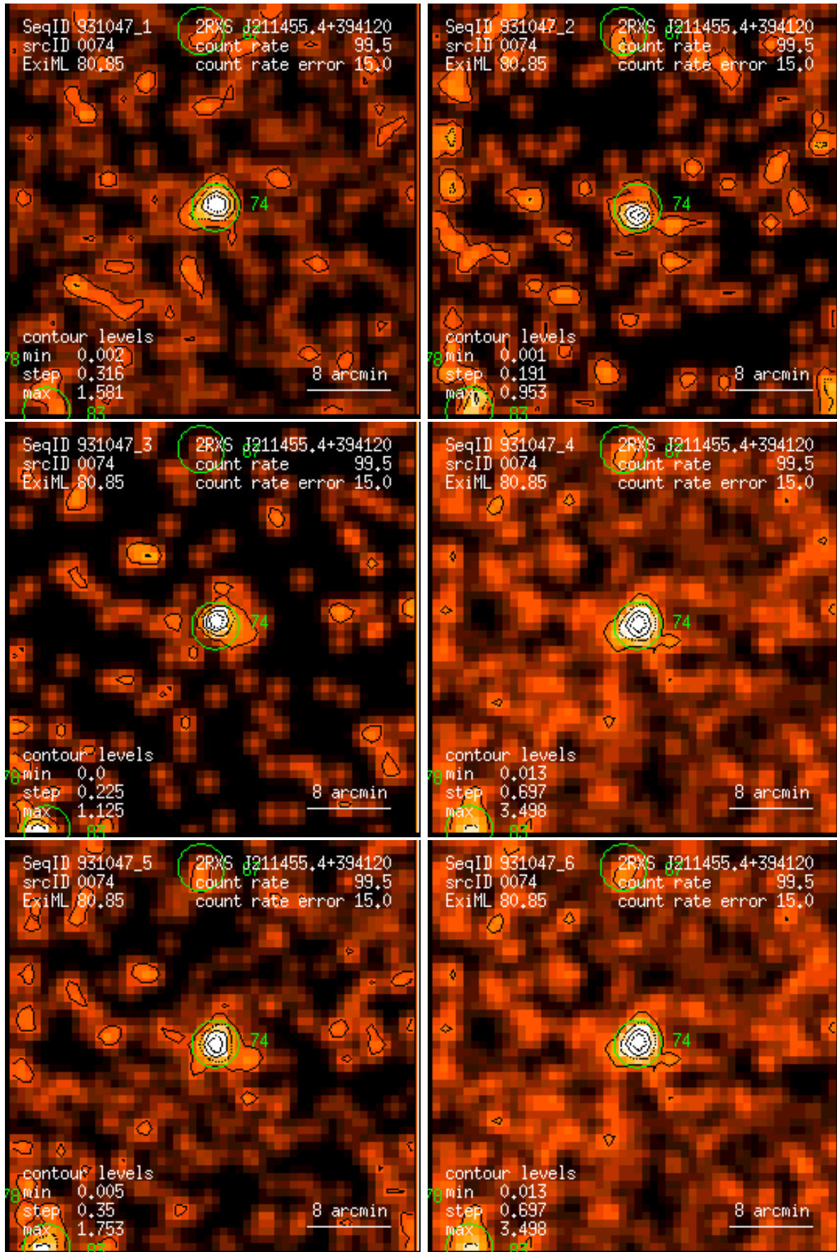
Figure 74: RASS 931047: detection 0074: band rate images, Gaussian filter: (1) PSPC channels 11 – 41, (2) 52 – 90, (3) 91 – 201, (4) 11 – 235, (5) 52 – 201, (6) 11 – 201. Broad band rates in counts/ks. Band rate contour levels in counts/ks/arcmin 2 .
