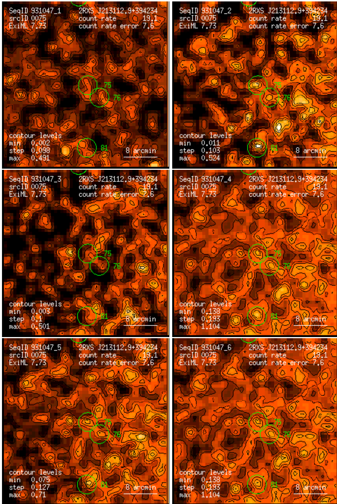
Figure 75: RASS 931047: detection 0075: band rate images, Gaussian filter: (1) PSPC channels 11 – 41, (2) 52 – 90, (3) 91 – 201, (4) 11 – 235, (5) 52 – 201, (6) 11 – 201. Broad band rates in counts/ks. Band rate contour levels in counts/ks/arcmin 2 .
