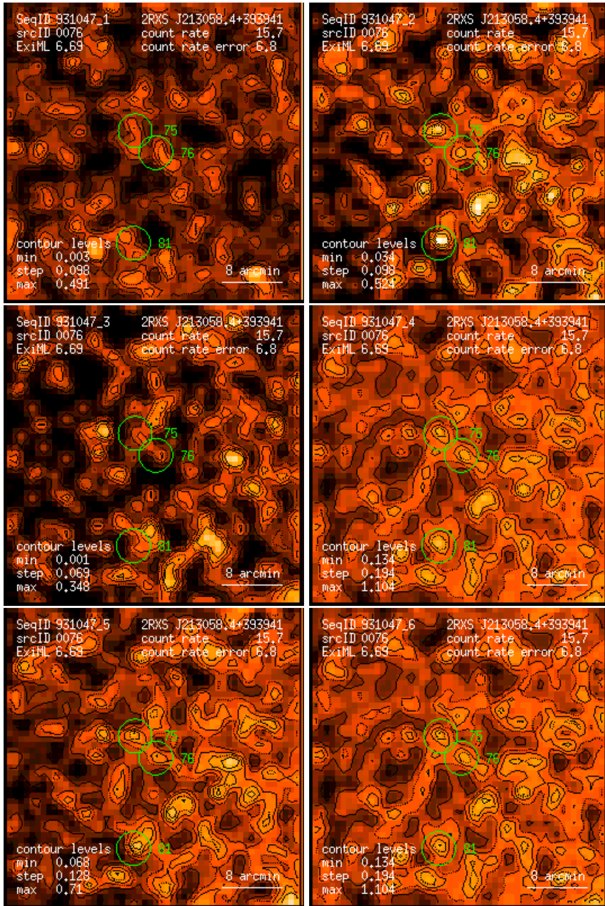
Figure 76: RASS 931047: detection 0076: band rate images, Gaussian filter: (1) PSPC channels 11 – 41, (2) 52 – 90, (3) 91 – 201, (4) 11 – 235, (5) 52 – 201, (6) 11 – 201. Broad band rates in counts/ks. Band rate contour levels in counts/ks/arcmin 2 .
