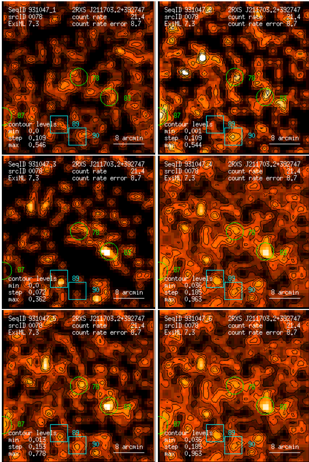
Figure 78: RASS 931047: detection 0078: band rate images, Gaussian filter: (1) PSPC channels 11 – 41, (2) 52 – 90, (3) 91 – 201, (4) 11 – 235, (5) 52 – 201, (6) 11 – 201. Broad band rates in counts/ks. Band rate contour levels in counts/ks/arcmin 2 .
