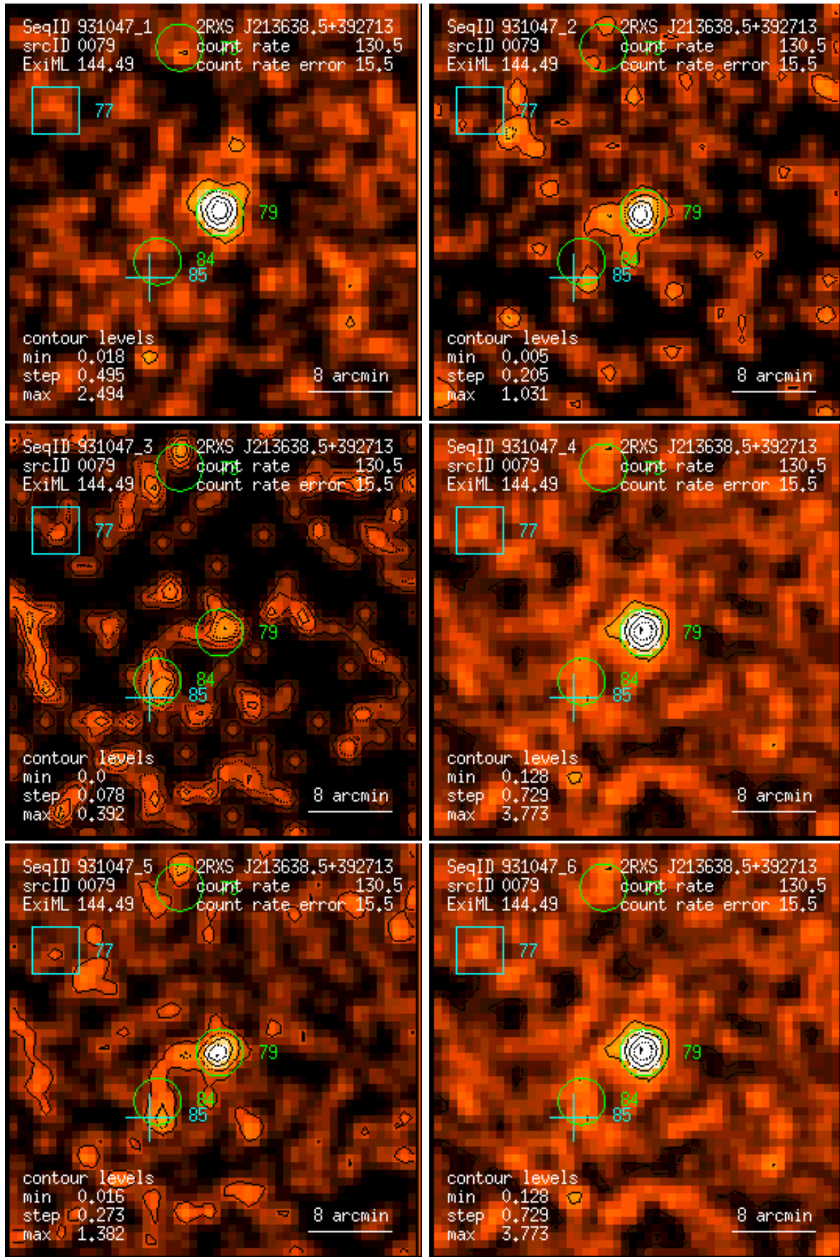
Figure 79: RASS 931047: detection 0079: band rate images, Gaussian filter: (1) PSPC channels 11 – 41, (2) 52 – 90, (3) 91 – 201, (4) 11 – 235, (5) 52 – 201, (6) 11 – 201. Broad band rates in counts/ks. Band rate contour levels in counts/ks/arcmin 2 .
