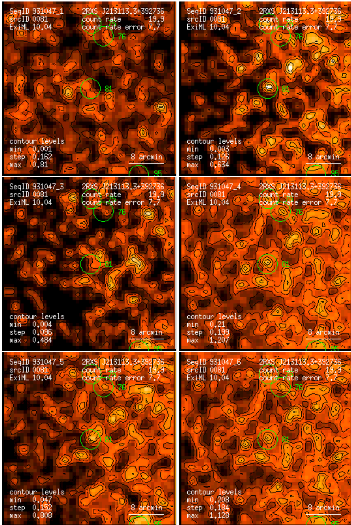
Figure 81: RASS 931047: detection 0081: band rate images, Gaussian filter: (1) PSPC channels 11 – 41, (2) 52 – 90, (3) 91 – 201, (4) 11 – 235, (5) 52 – 201, (6) 11 – 201. Broad band rates in counts/ks. Band rate contour levels in counts/ks/arcmin 2 .
