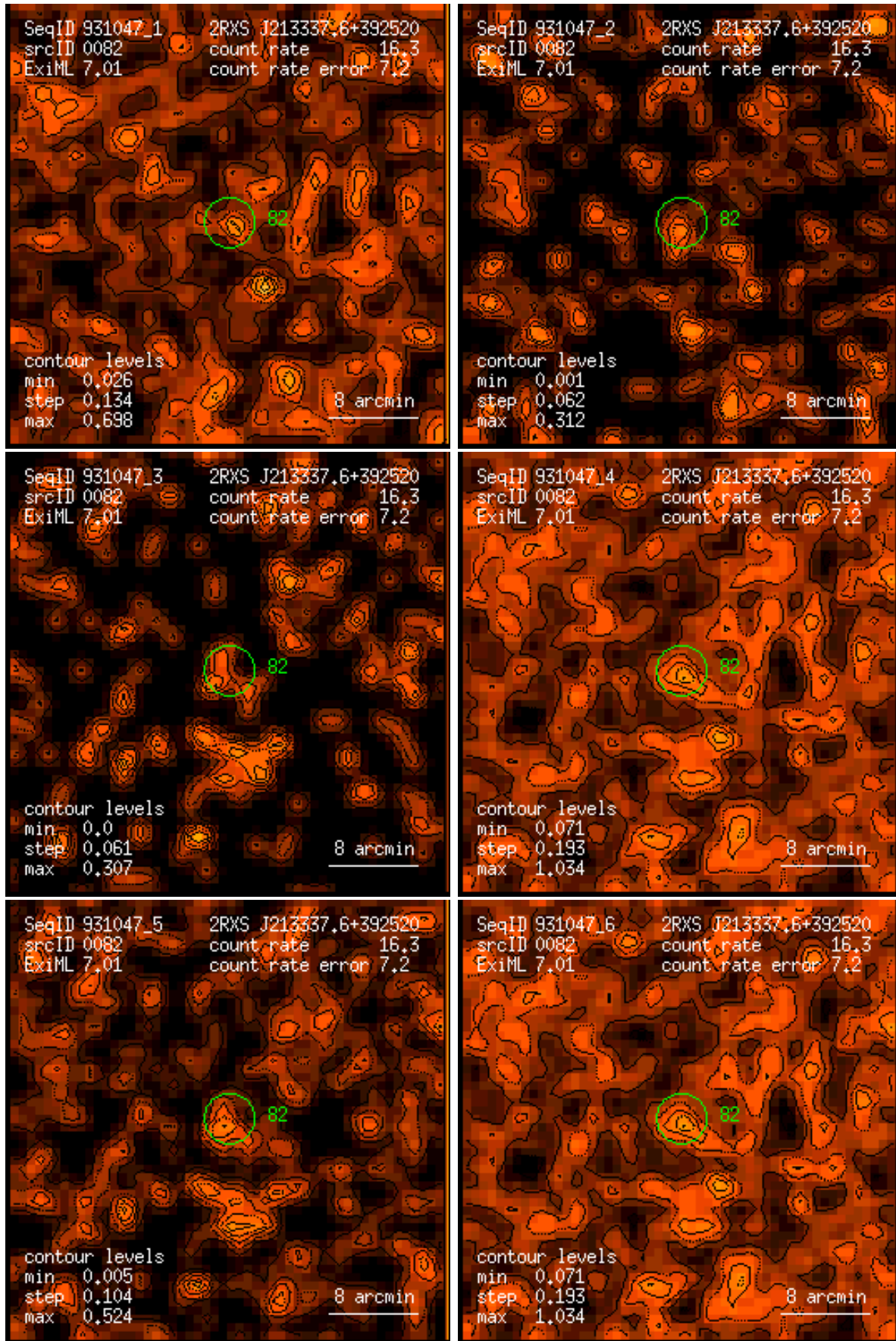
Figure 82: RASS 931047: detection 0082: band rate images, Gaussian filter: (1) PSPC channels 11 – 41, (2) 52 – 90, (3) 91 – 201, (4) 11 – 235, (5) 52 – 201, (6) 11 – 201. Broad band rates in counts/ks. Band rate contour levels in counts/ks/arcmin 2 .
