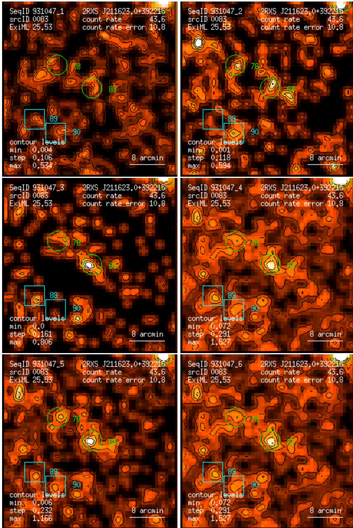
Figure 83: RASS 931047: detection 0083: band rate images, Gaussian filter: (1) PSPC channels 11 – 41, (2) 52 – 90, (3) 91 – 201, (4) 11 – 235, (5) 52 – 201, (6) 11 – 201. Broad band rates in counts/ks. Band rate contour levels in counts/ks/arcmin 2 .
