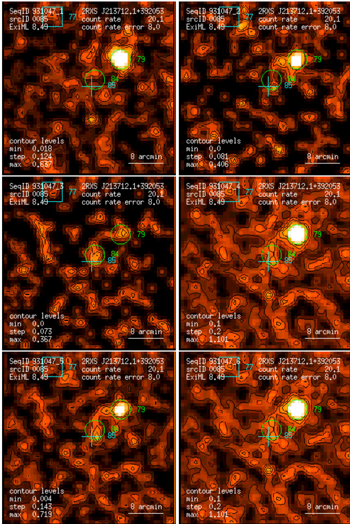
Figure 85: RASS 931047: detection 0085: band rate images, Gaussian filter: (1) PSPC channels 11 – 41, (2) 52 – 90, (3) 91 – 201, (4) 11 – 235, (5) 52 – 201, (6) 11 – 201. Broad band rates in counts/ks. Band rate contour levels in counts/ks/arcmin 2 .
