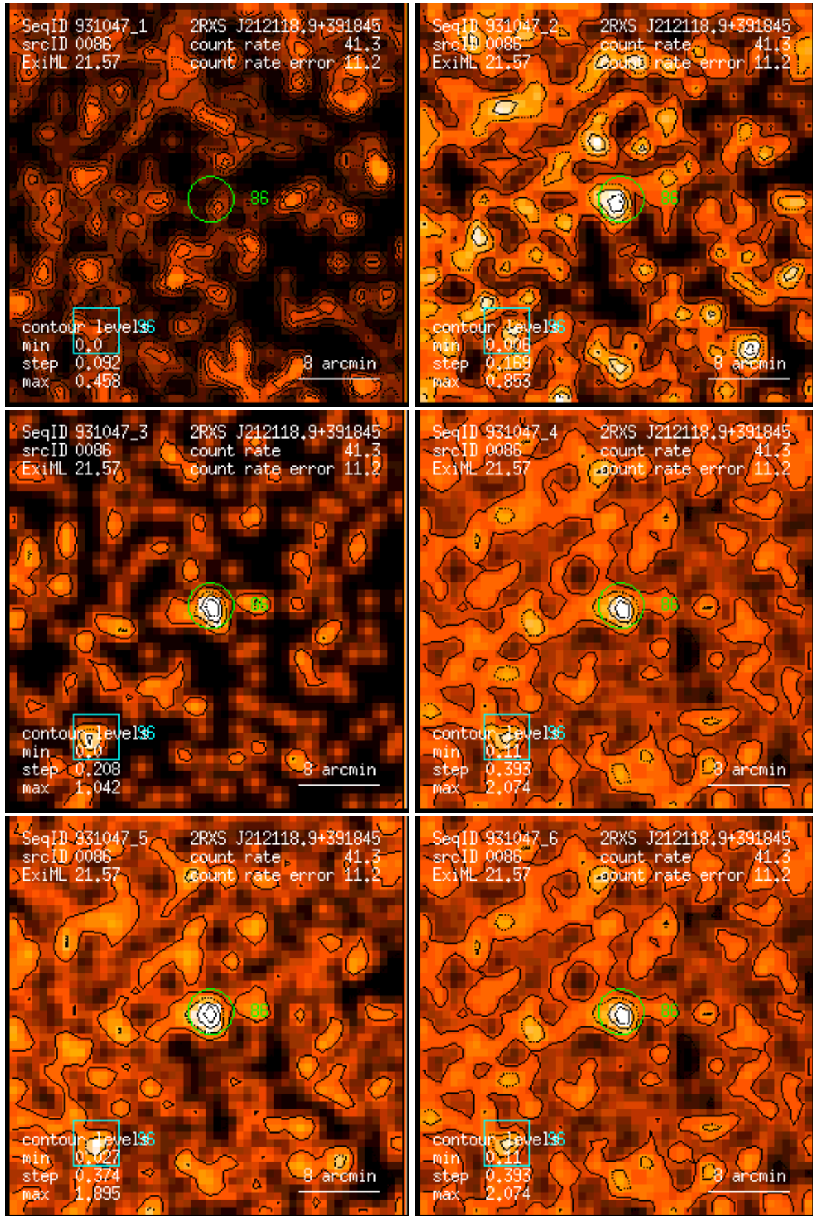
Figure 86: RASS 931047: detection 0086: band rate images, Gaussian filter: (1) PSPC channels 11 – 41, (2) 52 – 90, (3) 91 – 201, (4) 11 – 235, (5) 52 – 201, (6) 11 – 201. Broad band rates in counts/ks. Band rate contour levels in counts/ks/arcmin 2 .
