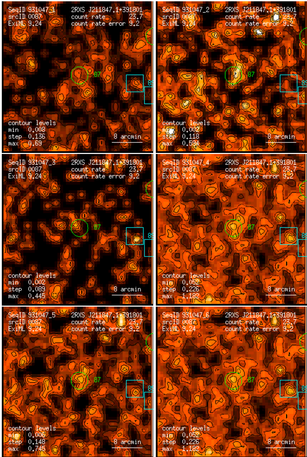
Figure 87: RASS 931047: detection 0087: band rate images, Gaussian filter: (1) PSPC channels 11 – 41, (2) 52 – 90, (3) 91 – 201, (4) 11 – 235, (5) 52 – 201, (6) 11 – 201. Broad band rates in counts/ks. Band rate contour levels in counts/ks/arcmin 2 .
