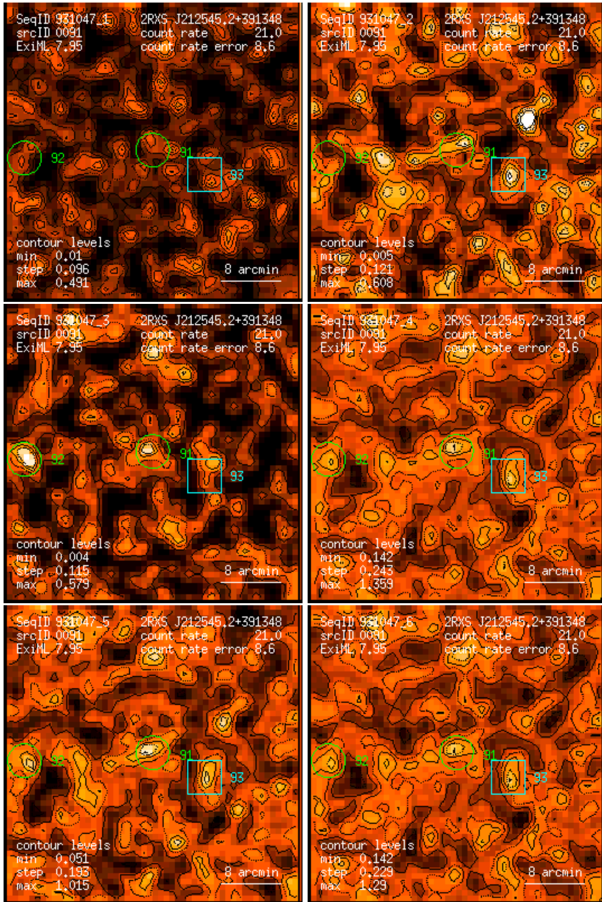
Figure 91: RASS 931047: detection 0091: band rate images, Gaussian filter: (1) PSPC channels 11 – 41, (2) 52 – 90, (3) 91 – 201, (4) 11 – 235, (5) 52 – 201, (6) 11 – 201. Broad band rates in counts/ks. Band rate contour levels in counts/ks/arcmin 2 .
