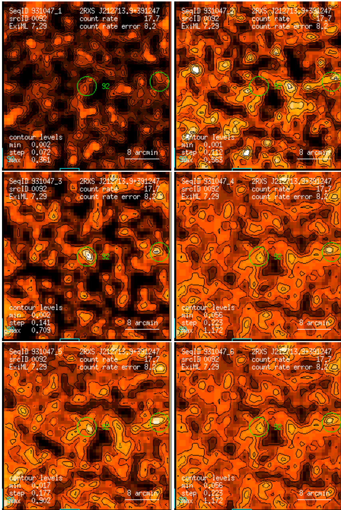
Figure 92: RASS 931047: detection 0092: band rate images, Gaussian filter: (1) PSPC channels 11 – 41, (2) 52 – 90, (3) 91 – 201, (4) 11 – 235, (5) 52 – 201, (6) 11 – 201. Broad band rates in counts/ks. Band rate contour levels in counts/ks/arcmin 2 .
