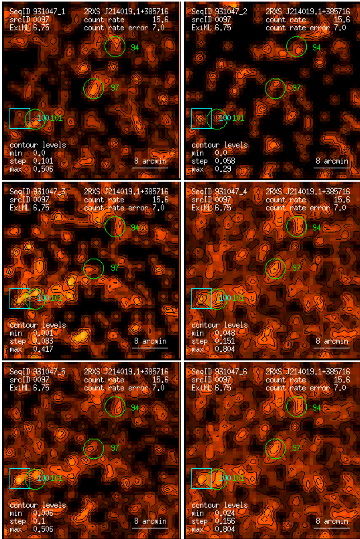
Figure 97: RASS 931047: detection 0097: band rate images, Gaussian filter: (1) PSPC channels 11 – 41, (2) 52 – 90, (3) 91 – 201, (4) 11 – 235, (5) 52 – 201, (6) 11 – 201. Broad band rates in counts/ks. Band rate contour levels in counts/ks/arcmin 2 .
