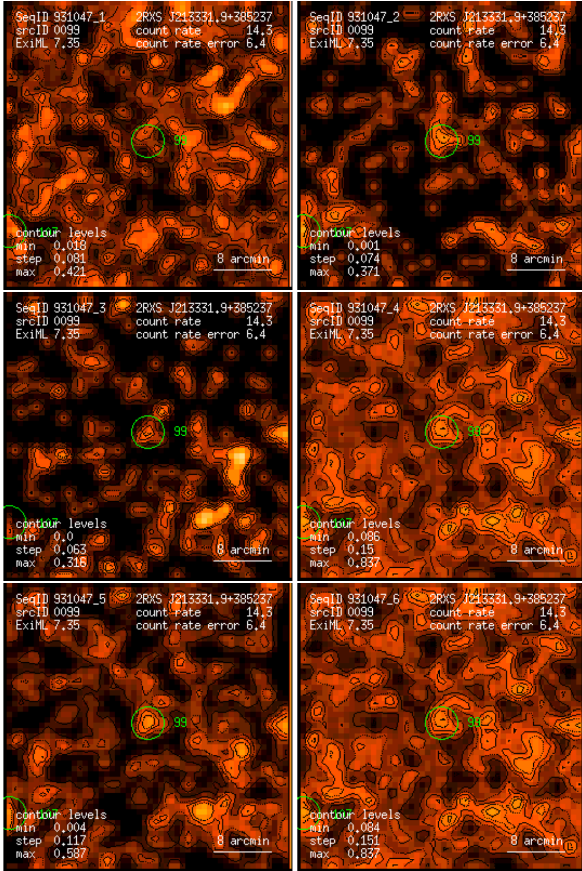
Figure 99: RASS 931047: detection 0099: band rate images, Gaussian filter: (1) PSPC channels 11 – 41, (2) 52 – 90, (3) 91 – 201, (4) 11 – 235, (5) 52 – 201, (6) 11 – 201. Broad band rates in counts/ks. Band rate contour levels in counts/ks/arcmin 2 .
