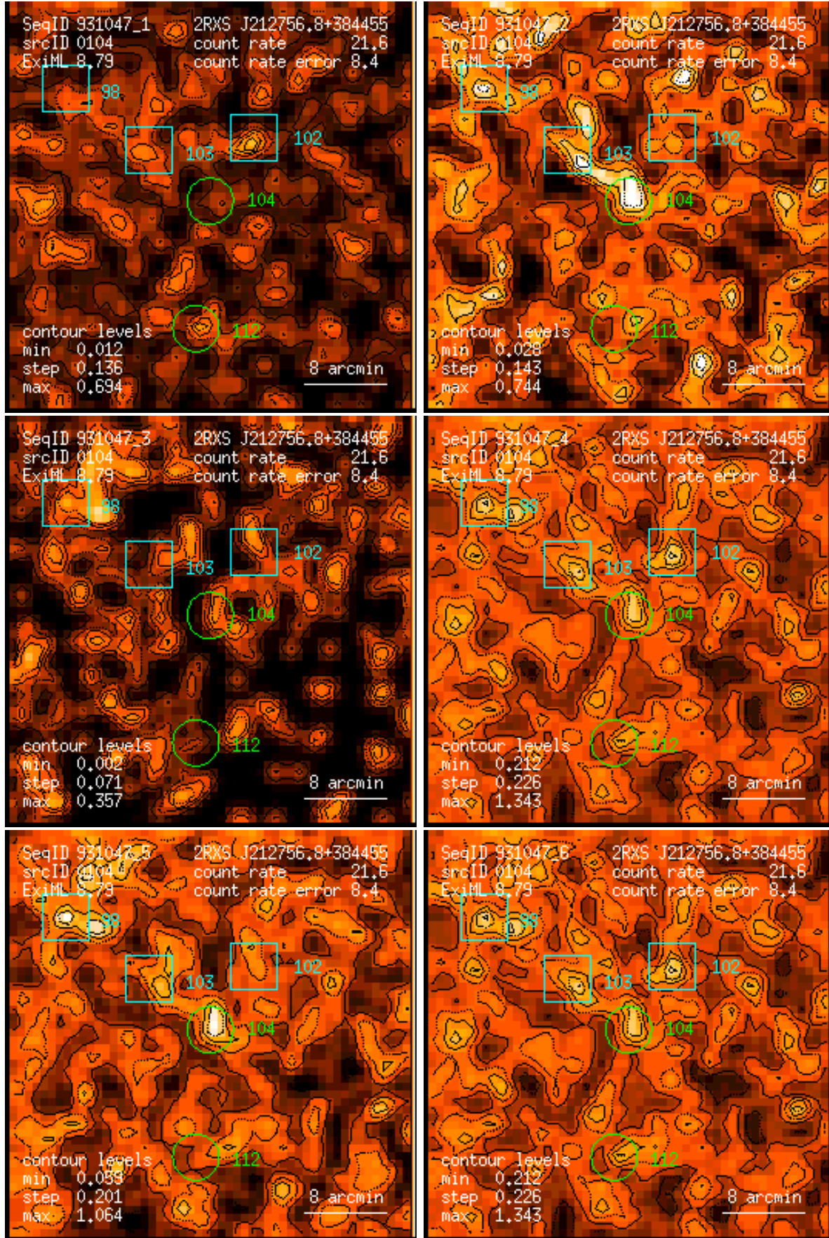
Figure 104: RASS 931047: detection 0104: band rate images, Gaussian filter: (1) PSPC channels 11 – 41, (2) 52 – 90, (3) 91 – 201, (4) 11 – 235, (5) 52 – 201, (6) 11 – 201. Broad band rates in counts/ks. Band rate contour levels in counts/ks/arcmin 2 .
