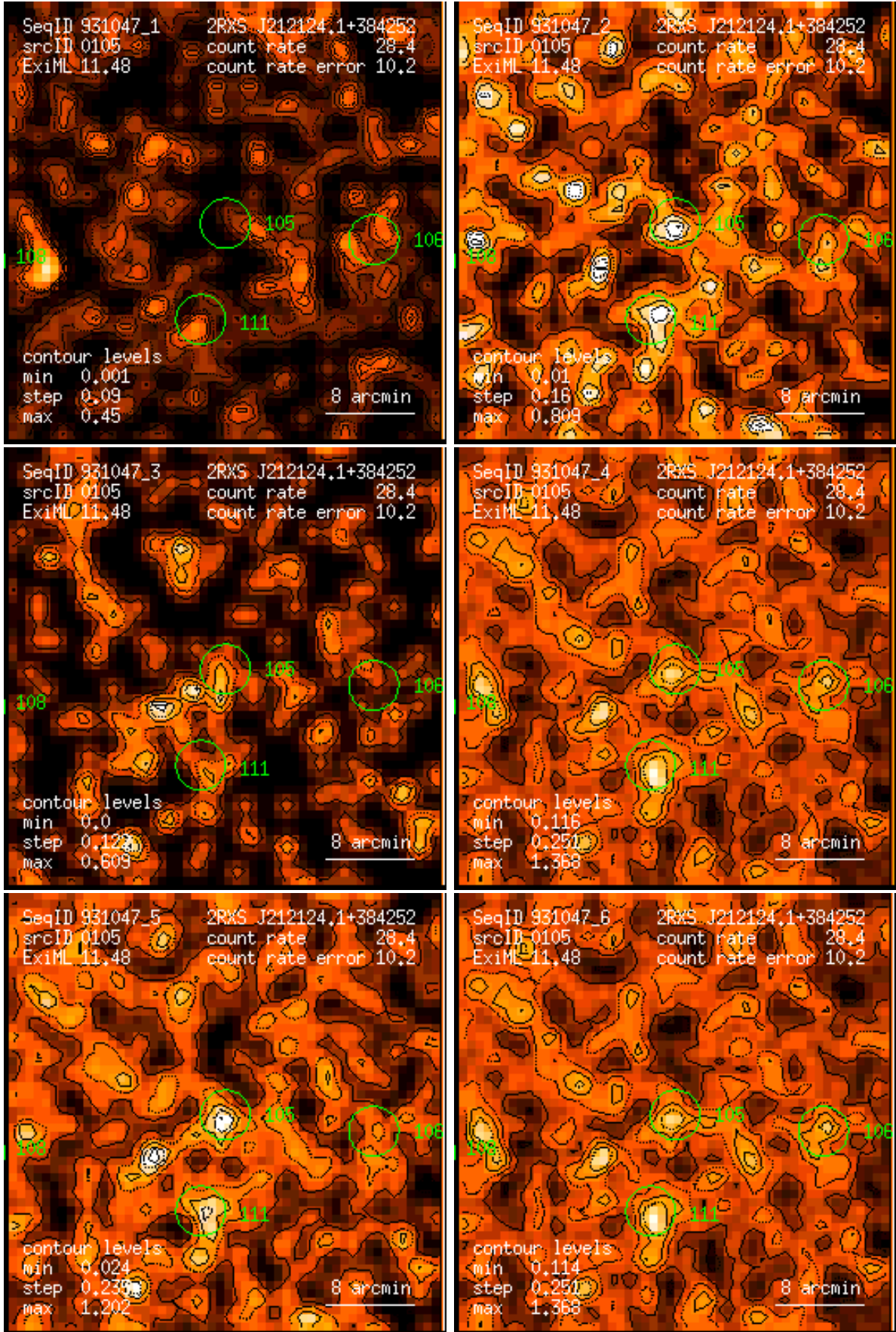
Figure 105: RASS 931047: detection 0105: band rate images, Gaussian filter: (1) PSPC channels 11 – 41, (2) 52 – 90, (3) 91 – 201, (4) 11 – 235, (5) 52 – 201, (6) 11 – 201. Broad band rates in counts/ks. Band rate contour levels in counts/ks/arcmin 2 .
