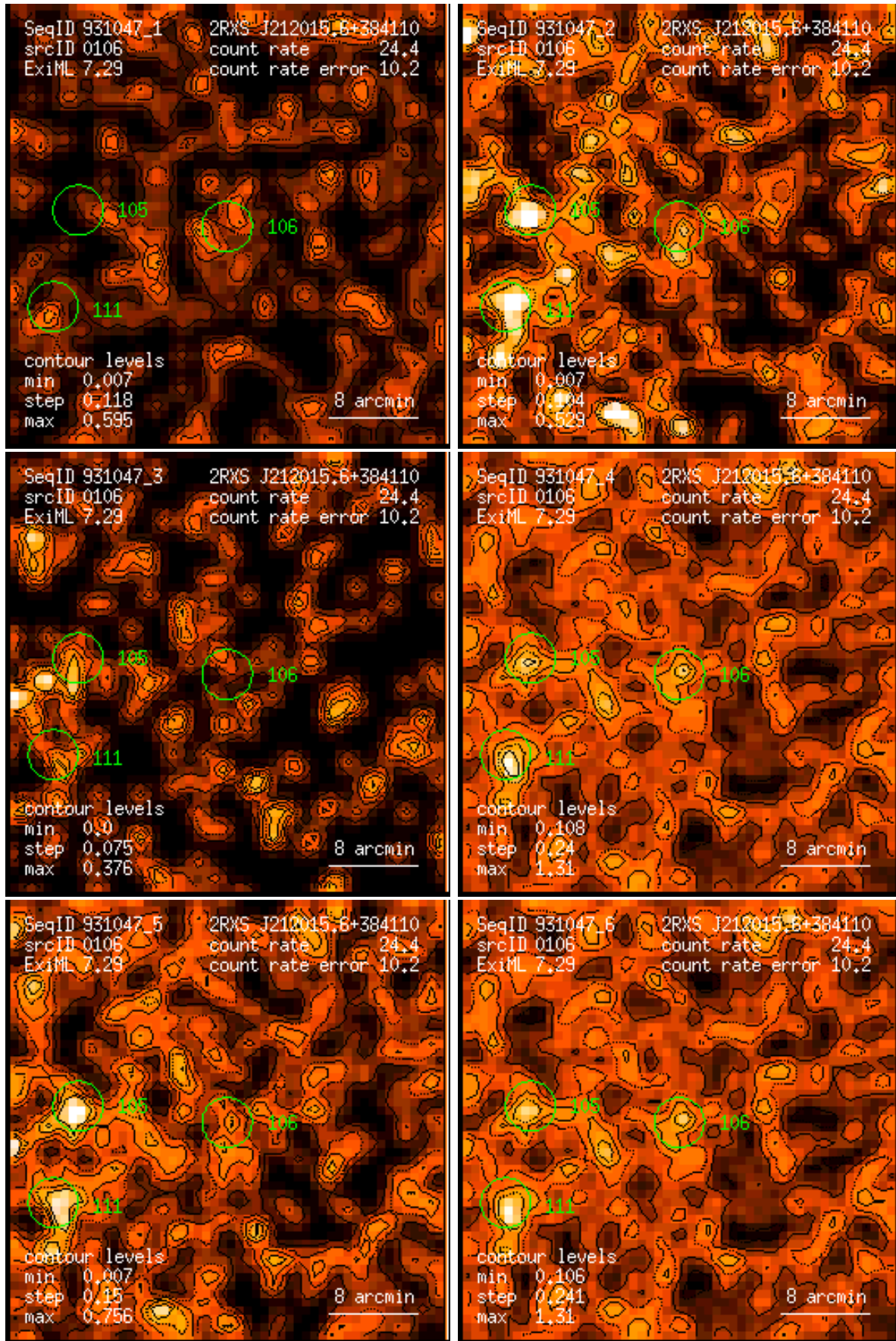
Figure 106: RASS 931047: detection 0106: band rate images, Gaussian filter: (1) PSPC channels 11 – 41, (2) 52 – 90, (3) 91 – 201, (4) 11 – 235, (5) 52 – 201, (6) 11 – 201. Broad band rates in counts/ks. Band rate contour levels in counts/ks/arcmin 2 .
