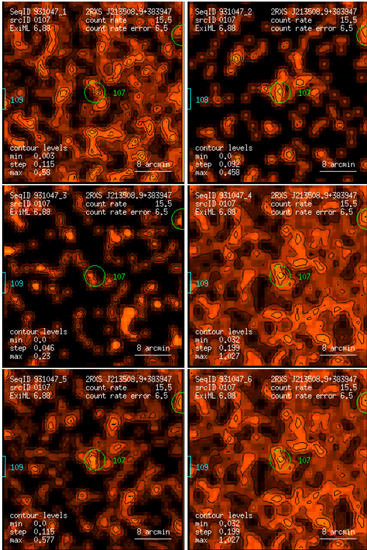
Figure 107: RASS 931047: detection 0107: band rate images, Gaussian filter: (1) PSPC channels 11 – 41, (2) 52 – 90, (3) 91 – 201, (4) 11 – 235, (5) 52 – 201, (6) 11 – 201. Broad band rates in counts/ks. Band rate contour levels in counts/ks/arcmin 2 .
