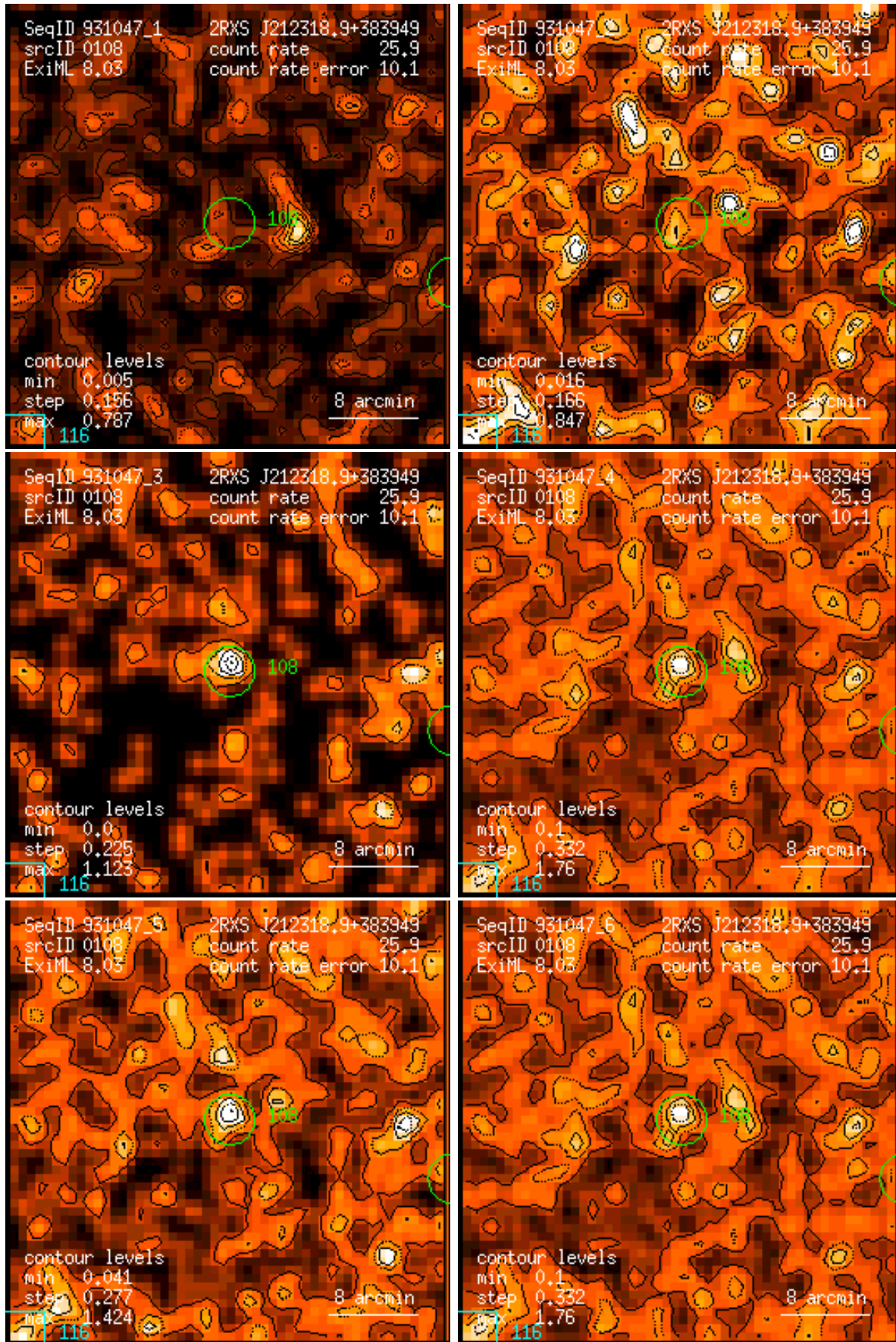
Figure 108: RASS 931047: detection 0108: band rate images, Gaussian filter: (1) PSPC channels 11 – 41, (2) 52 – 90, (3) 91 – 201, (4) 11 – 235, (5) 52 – 201, (6) 11 – 201. Broad band rates in counts/ks. Band rate contour levels in counts/ks/arcmin 2 .
