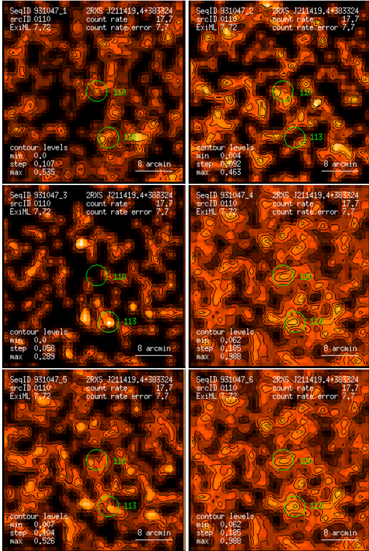
Figure 110: RASS 931047: detection 0110: band rate images, Gaussian filter: (1) PSPC channels 11 – 41, (2) 52 – 90, (3) 91 – 201, (4) 11 – 235, (5) 52 – 201, (6) 11 – 201. Broad band rates in counts/ks. Band rate contour levels in counts/ks/arcmin 2 .
