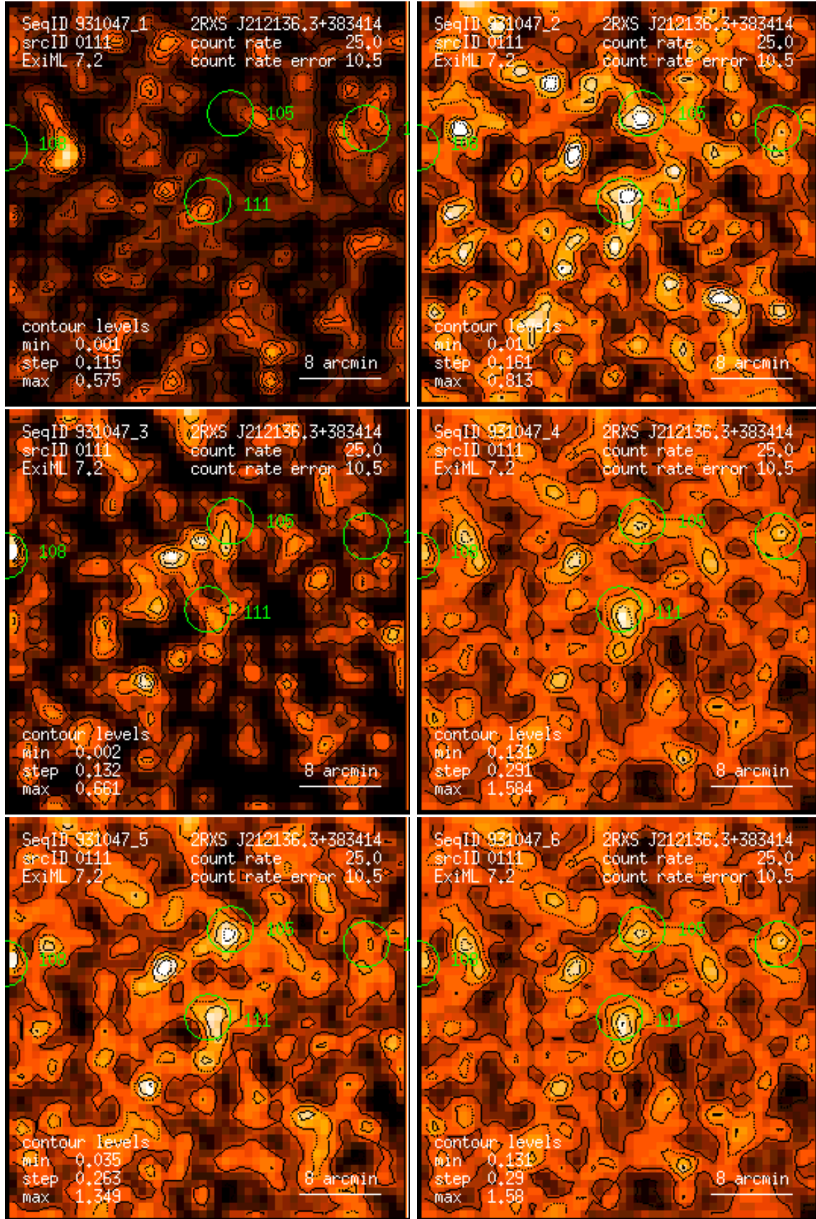
Figure 111: RASS 931047: detection 0111: band rate images, Gaussian filter: (1) PSPC channels 11 – 41, (2) 52 – 90, (3) 91 – 201, (4) 11 – 235, (5) 52 – 201, (6) 11 – 201. Broad band rates in counts/ks. Band rate contour levels in counts/ks/arcmin 2 .
