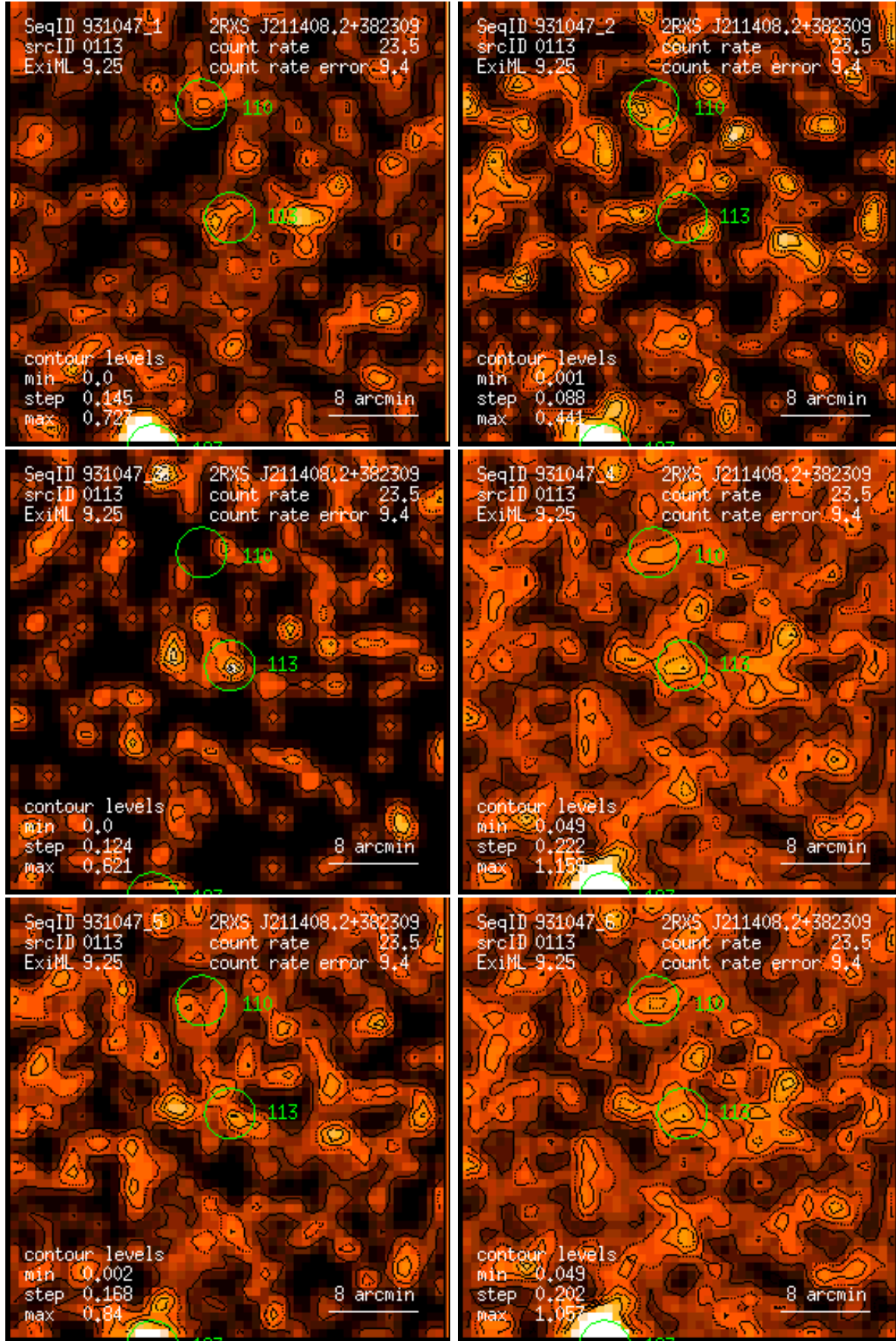
Figure 113: RASS 931047: detection 0113: band rate images, Gaussian filter: (1) PSPC channels 11 – 41, (2) 52 – 90, (3) 91 – 201, (4) 11 – 235, (5) 52 – 201, (6) 11 – 201. Broad band rates in counts/ks. Band rate contour levels in counts/ks/arcmin 2 .
