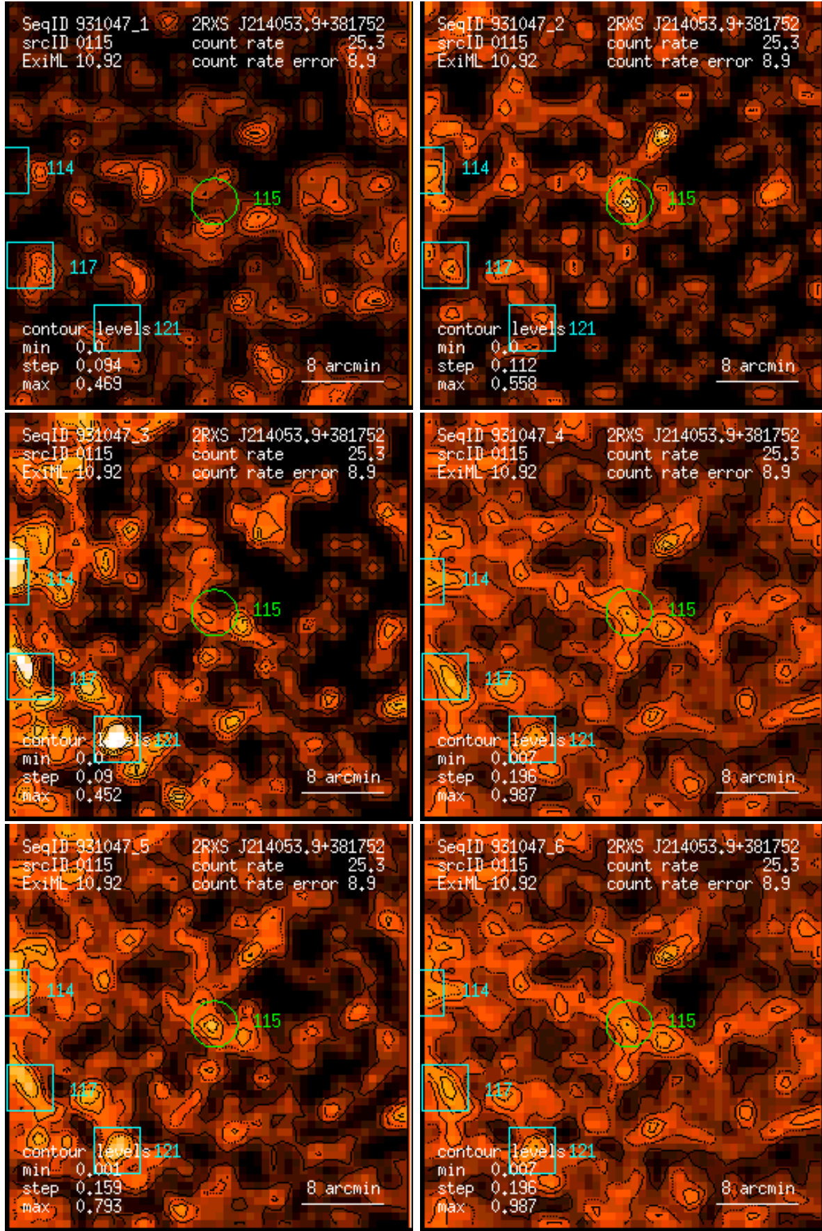
Figure 115: RASS 931047: detection 0115: band rate images, Gaussian filter: (1) PSPC channels 11 – 41, (2) 52 – 90, (3) 91 – 201, (4) 11 – 235, (5) 52 – 201, (6) 11 – 201. Broad band rates in counts/ks. Band rate contour levels in counts/ks/arcmin 2 .
