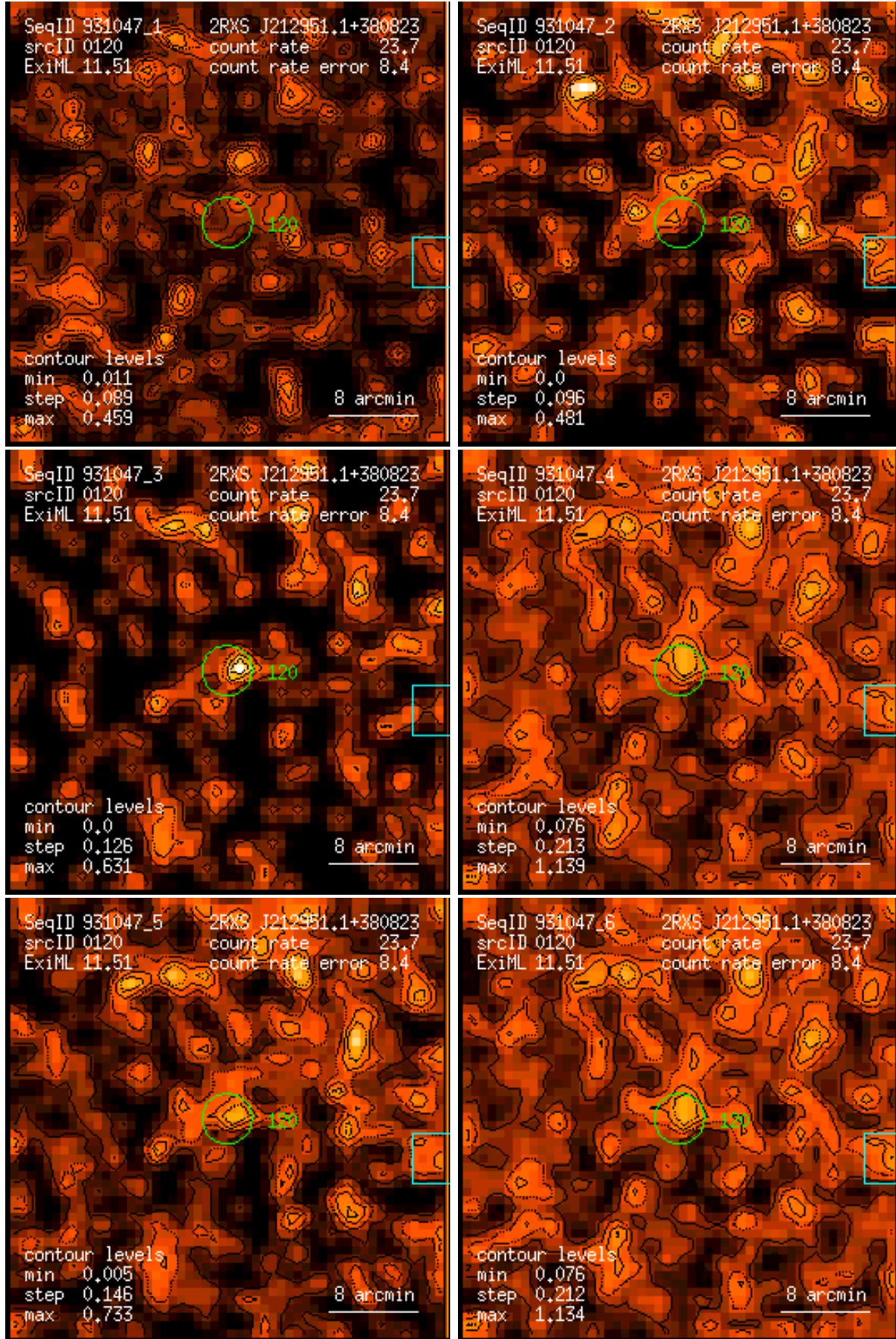
Figure 120: RASS 931047: detection 0120: band rate images, Gaussian filter: (1) PSPC channels 11 – 41, (2) 52 – 90, (3) 91 – 201, (4) 11 – 235, (5) 52 – 201, (6) 11 – 201. Broad band rates in counts/ks. Band rate contour levels in counts/ks/arcmin 2 .
