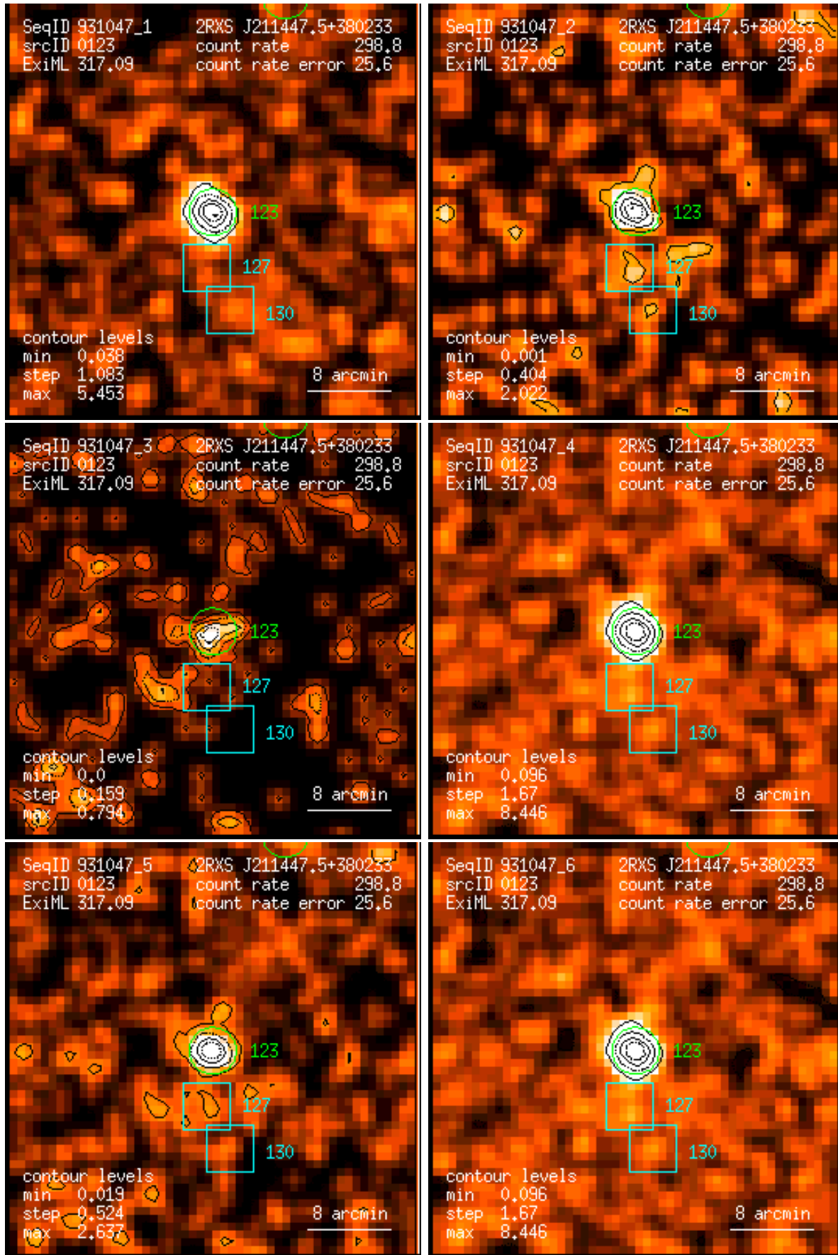
Figure 123: RASS 931047: detection 0123: band rate images, Gaussian filter: (1) PSPC channels 11 – 41, (2) 52 – 90, (3) 91 – 201, (4) 11 – 235, (5) 52 – 201, (6) 11 – 201. Broad band rates in counts/ks. Band rate contour levels in counts/ks/arcmin 2 .
