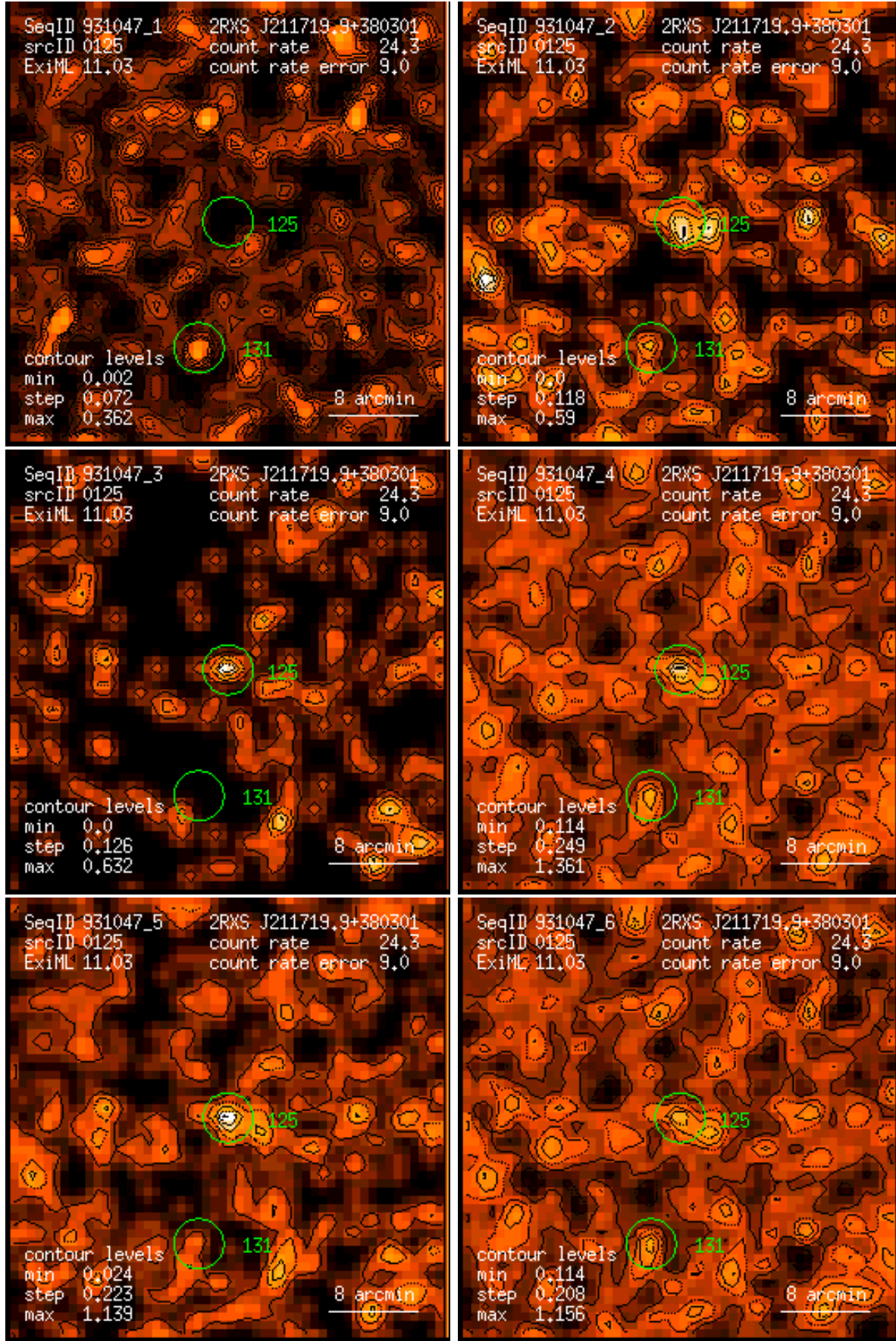
Figure 125: RASS 931047: detection 0125: band rate images, Gaussian filter: (1) PSPC channels 11 – 41, (2) 52 – 90, (3) 91 – 201, (4) 11 – 235, (5) 52 – 201, (6) 11 – 201. Broad band rates in counts/ks. Band rate contour levels in counts/ks/arcmin 2 .
