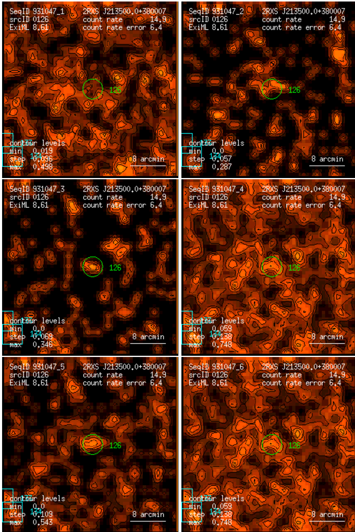
Figure 126: RASS 931047: detection 0126: band rate images, Gaussian filter: (1) PSPC channels 11 – 41, (2) 52 – 90, (3) 91 – 201, (4) 11 – 235, (5) 52 – 201, (6) 11 – 201. Broad band rates in counts/ks. Band rate contour levels in counts/ks/arcmin 2 .
