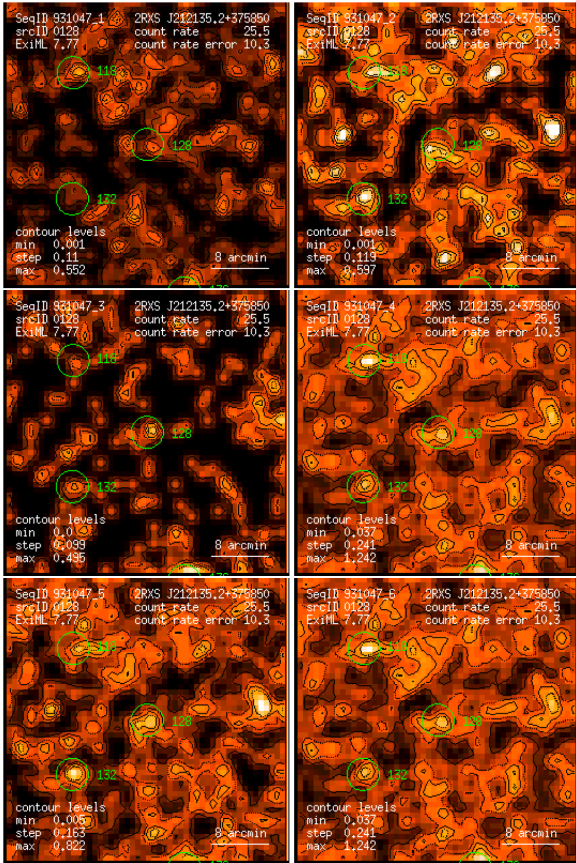
Figure 128: RASS 931047: detection 0128: band rate images, Gaussian filter: (1) PSPC channels 11 – 41, (2) 52 – 90, (3) 91 – 201, (4) 11 – 235, (5) 52 – 201, (6) 11 – 201. Broad band rates in counts/ks. Band rate contour levels in counts/ks/arcmin 2 .
