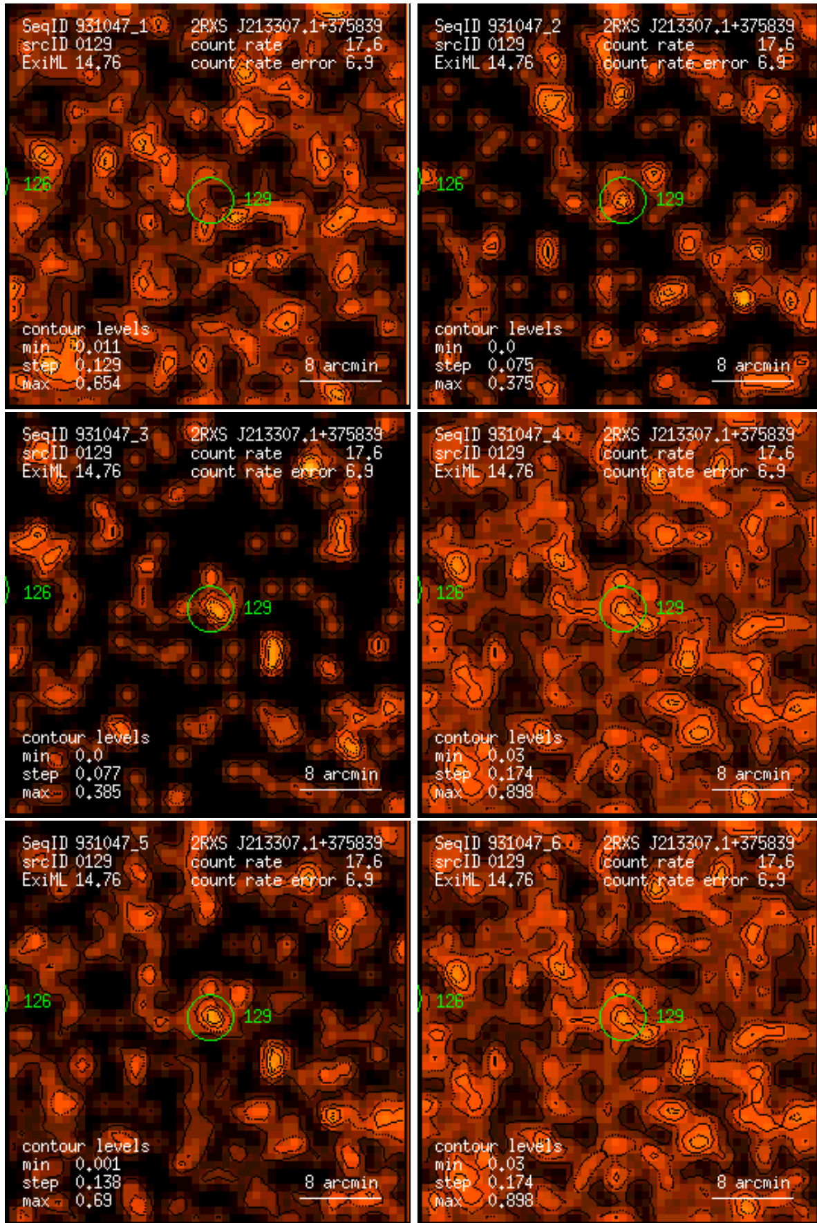
Figure 129: RASS 931047: detection 0129: band rate images, Gaussian filter: (1) PSPC channels 11 – 41, (2) 52 – 90, (3) 91 – 201, (4) 11 – 235, (5) 52 – 201, (6) 11 – 201. Broad band rates in counts/ks. Band rate contour levels in counts/ks/arcmin 2 .
