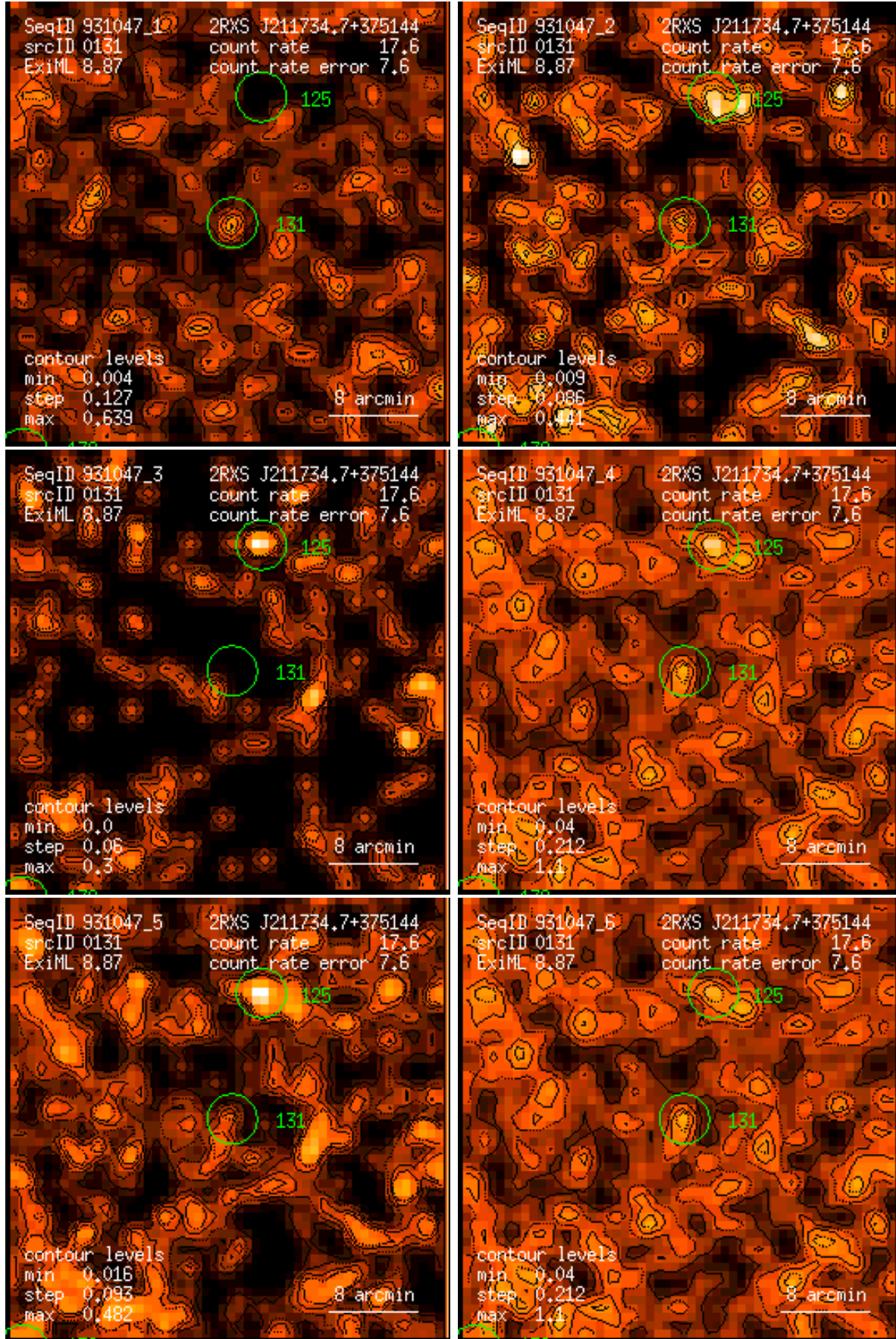
Figure 131: RASS 931047: detection 0131: band rate images, Gaussian filter: (1) PSPC channels 11 – 41, (2) 52 – 90, (3) 91 – 201, (4) 11 – 235, (5) 52 – 201, (6) 11 – 201. Broad band rates in counts/ks. Band rate contour levels in counts/ks/arcmin 2 .
