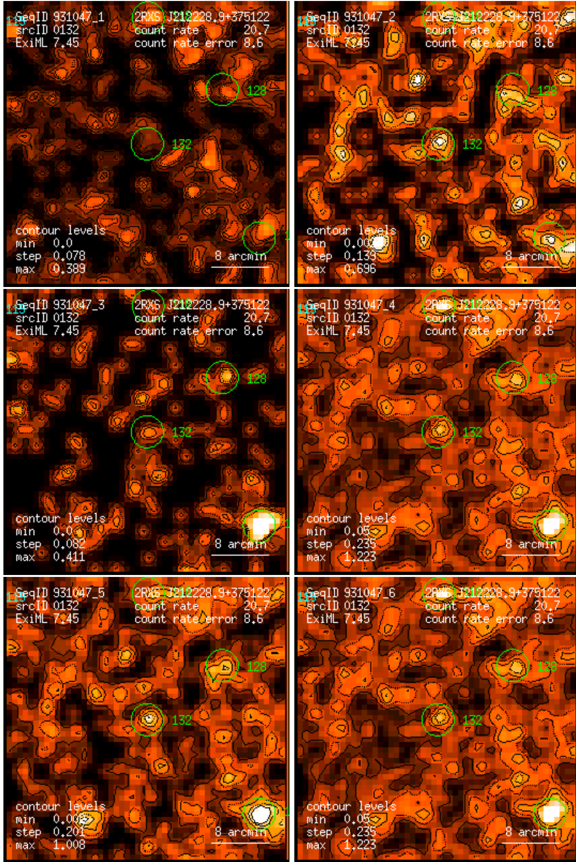
Figure 132: RASS 931047: detection 0132: band rate images, Gaussian filter: (1) PSPC channels 11 – 41, (2) 52 – 90, (3) 91 – 201, (4) 11 – 235, (5) 52 – 201, (6) 11 – 201. Broad band rates in counts/ks. Band rate contour levels in counts/ks/arcmin 2 .
