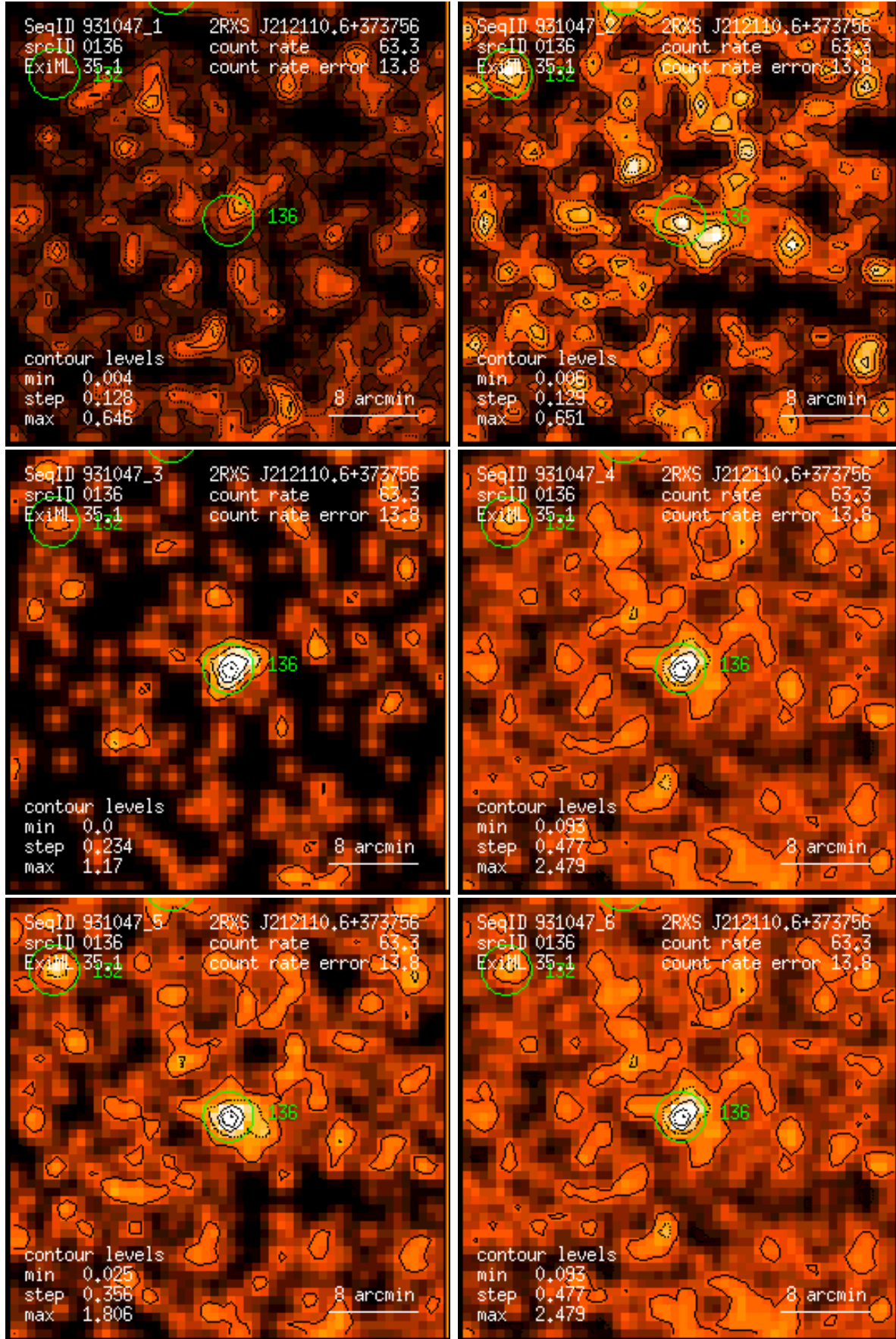
Figure 136: RASS 931047: detection 0136: band rate images, Gaussian filter: (1) PSPC channels 11 – 41, (2) 52 – 90, (3) 91 – 201, (4) 11 – 235, (5) 52 – 201, (6) 11 – 201. Broad band rates in counts/ks. Band rate contour levels in counts/ks/arcmin 2 .
