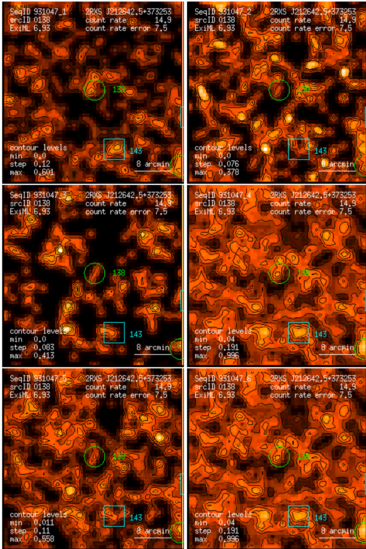
Figure 138: RASS 931047: detection 0138: band rate images, Gaussian filter: (1) PSPC channels 11 – 41, (2) 52 – 90, (3) 91 – 201, (4) 11 – 235, (5) 52 – 201, (6) 11 – 201. Broad band rates in counts/ks. Band rate contour levels in counts/ks/arcmin 2 .
