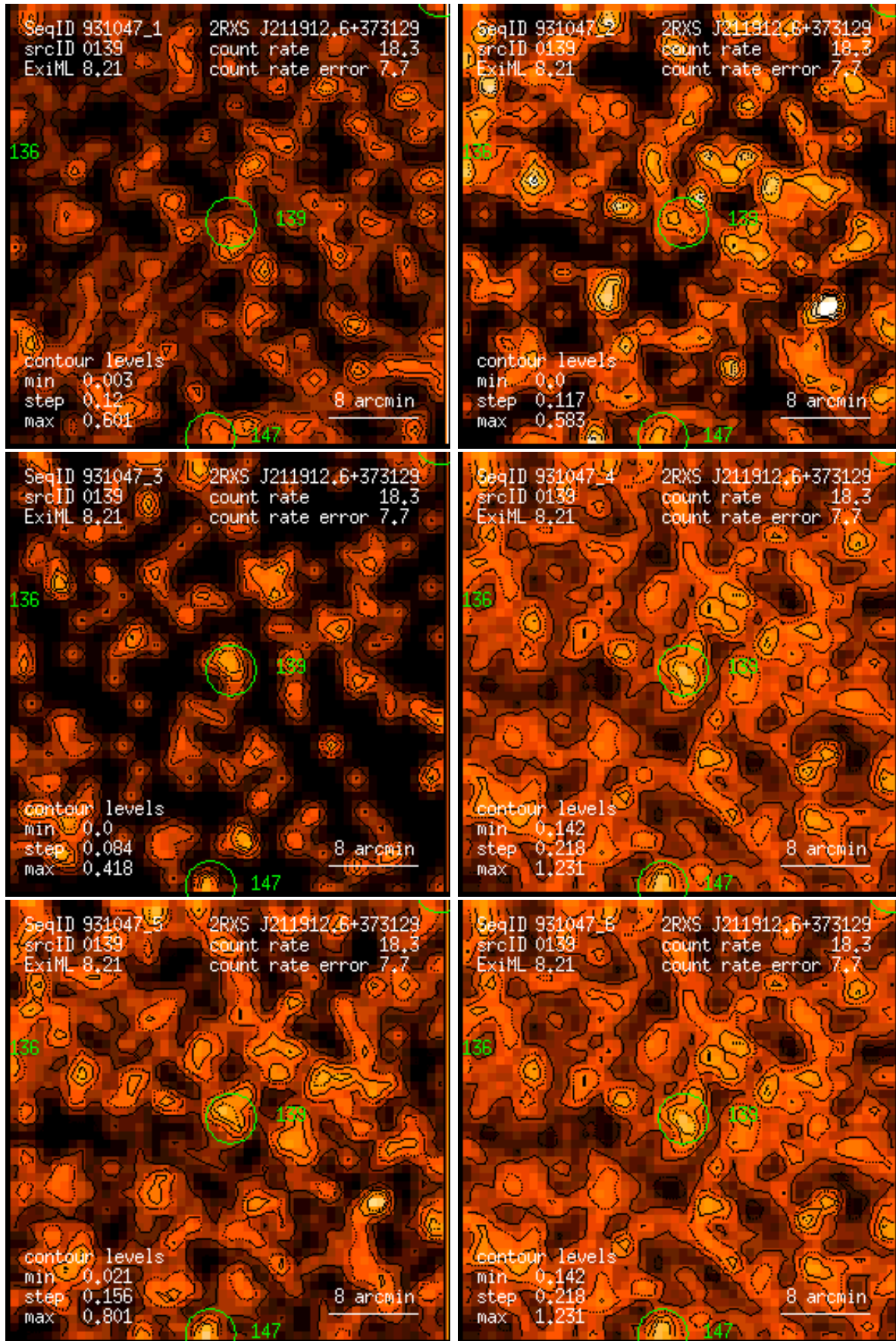
Figure 139: RASS 931047: detection 0139: band rate images, Gaussian filter: (1) PSPC channels 11 – 41, (2) 52 – 90, (3) 91 – 201, (4) 11 – 235, (5) 52 – 201, (6) 11 – 201. Broad band rates in counts/ks. Band rate contour levels in counts/ks/arcmin 2 .
