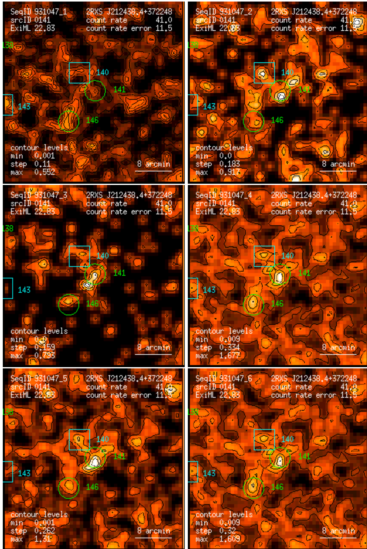
Figure 141: RASS 931047: detection 0141: band rate images, Gaussian filter: (1) PSPC channels 11 – 41, (2) 52 – 90, (3) 91 – 201, (4) 11 – 235, (5) 52 – 201, (6) 11 – 201. Broad band rates in counts/ks. Band rate contour levels in counts/ks/arcmin 2 .
