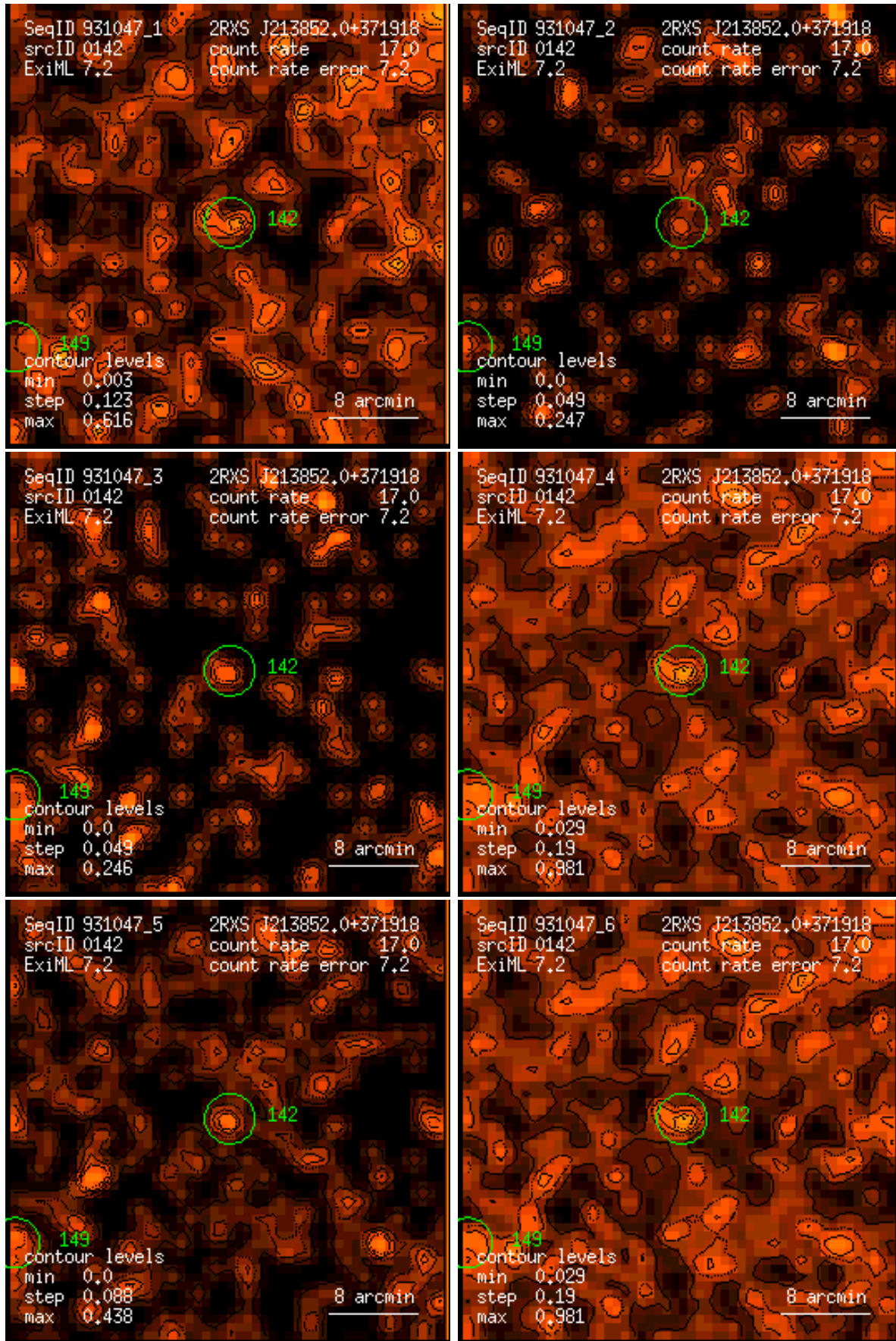
Figure 142: RASS 931047: detection 0142: band rate images, Gaussian filter: (1) PSPC channels 11 – 41, (2) 52 – 90, (3) 91 – 201, (4) 11 – 235, (5) 52 – 201, (6) 11 – 201. Broad band rates in counts/ks. Band rate contour levels in counts/ks/arcmin 2 .
