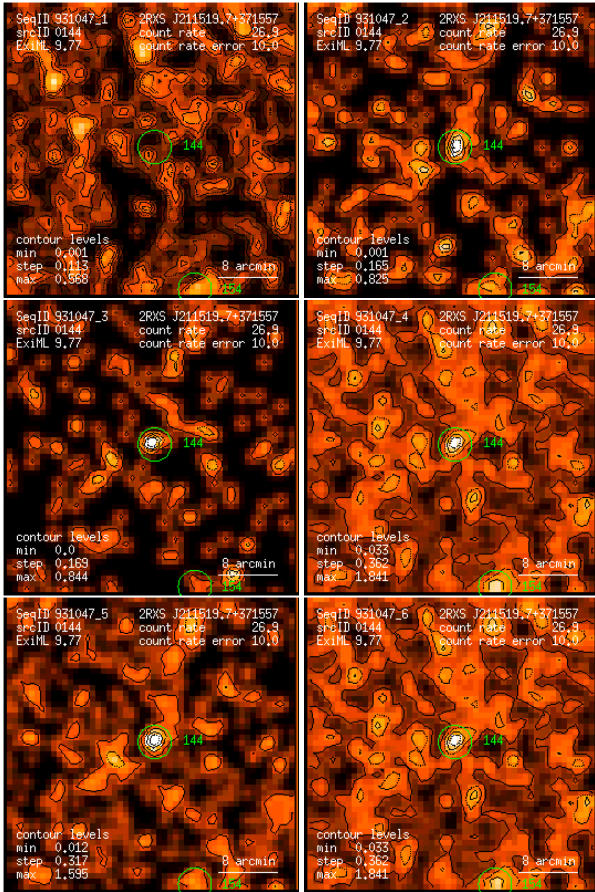
Figure 144: RASS 931047: detection 0144: band rate images, Gaussian filter: (1) PSPC channels 11 – 41, (2) 52 – 90, (3) 91 – 201, (4) 11 – 235, (5) 52 – 201, (6) 11 – 201. Broad band rates in counts/ks. Band rate contour levels in counts/ks/arcmin 2 .
