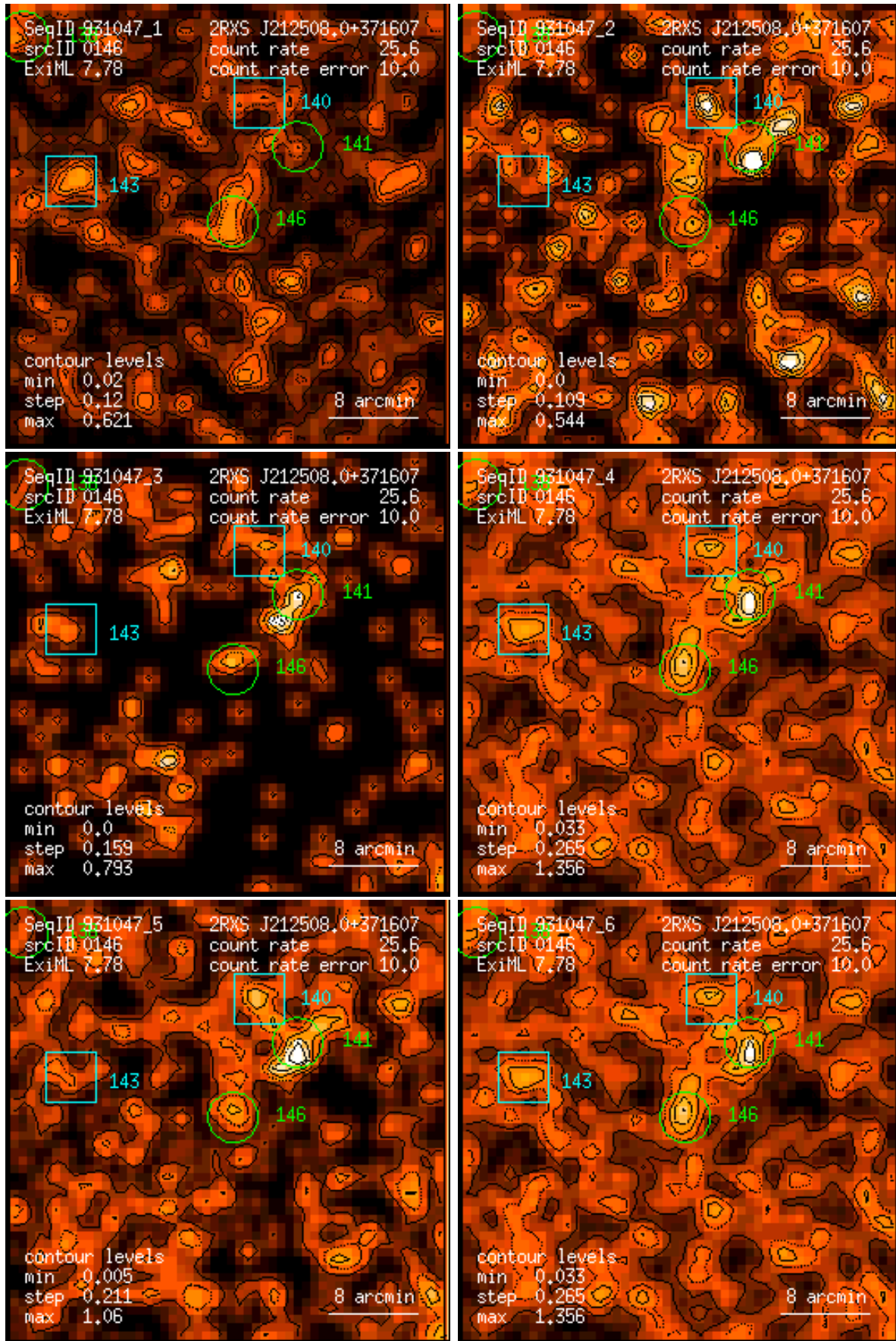
Figure 146: RASS 931047: detection 0146: band rate images, Gaussian filter: (1) PSPC channels 11 – 41, (2) 52 – 90, (3) 91 – 201, (4) 11 – 235, (5) 52 – 201, (6) 11 – 201. Broad band rates in counts/ks. Band rate contour levels in counts/ks/arcmin 2 .
