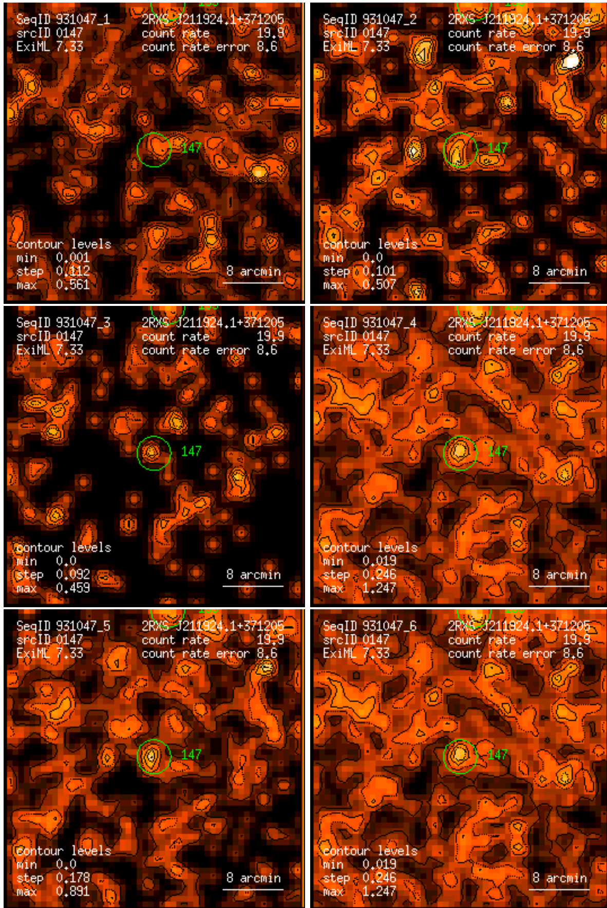
Figure 147: RASS 931047: detection 0147: band rate images, Gaussian filter: (1) PSPC channels 11 – 41, (2) 52 – 90, (3) 91 – 201, (4) 11 – 235, (5) 52 – 201, (6) 11 – 201. Broad band rates in counts/ks. Band rate contour levels in counts/ks/arcmin 2 .
