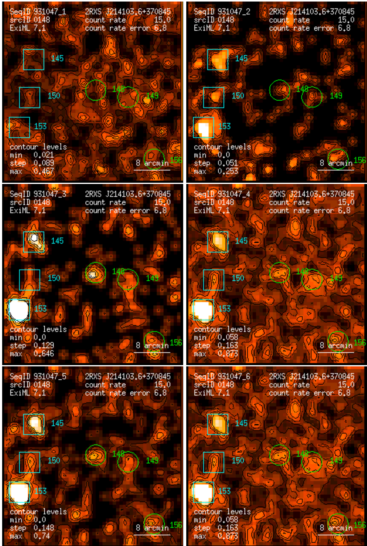
Figure 148: RASS 931047: detection 0148: band rate images, Gaussian filter: (1) PSPC channels 11 – 41, (2) 52 – 90, (3) 91 – 201, (4) 11 – 235, (5) 52 – 201, (6) 11 – 201. Broad band rates in counts/ks. Band rate contour levels in counts/ks/arcmin 2 .
