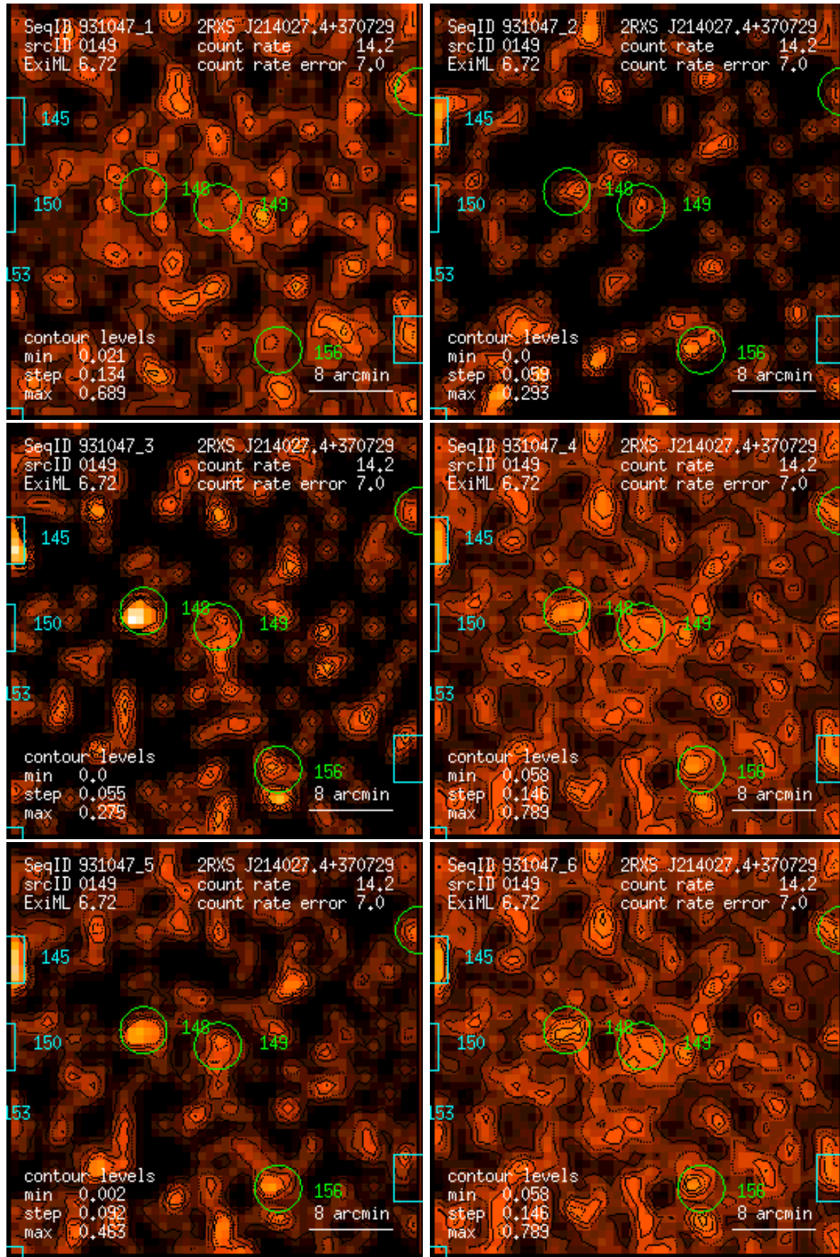
Figure 149: RASS 931047: detection 0149: band rate images, Gaussian filter: (1) PSPC channels 11 – 41, (2) 52 – 90, (3) 91 – 201, (4) 11 – 235, (5) 52 – 201, (6) 11 – 201. Broad band rates in counts/ks. Band rate contour levels in counts/ks/arcmin 2 .
