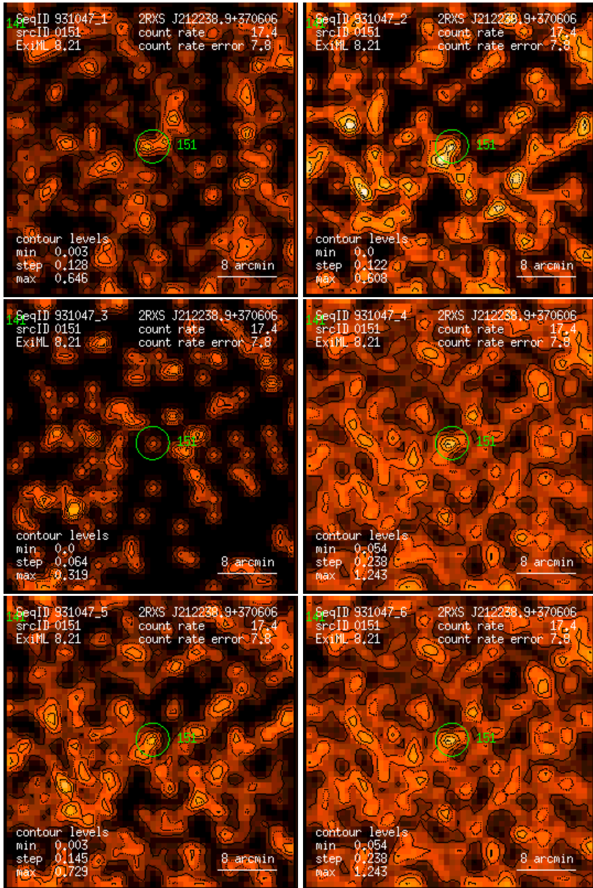
Figure 151: RASS 931047: detection 0151: band rate images, Gaussian filter: (1) PSPC channels 11 – 41, (2) 52 – 90, (3) 91 – 201, (4) 11 – 235, (5) 52 – 201, (6) 11 – 201. Broad band rates in counts/ks. Band rate contour levels in counts/ks/arcmin 2 .
