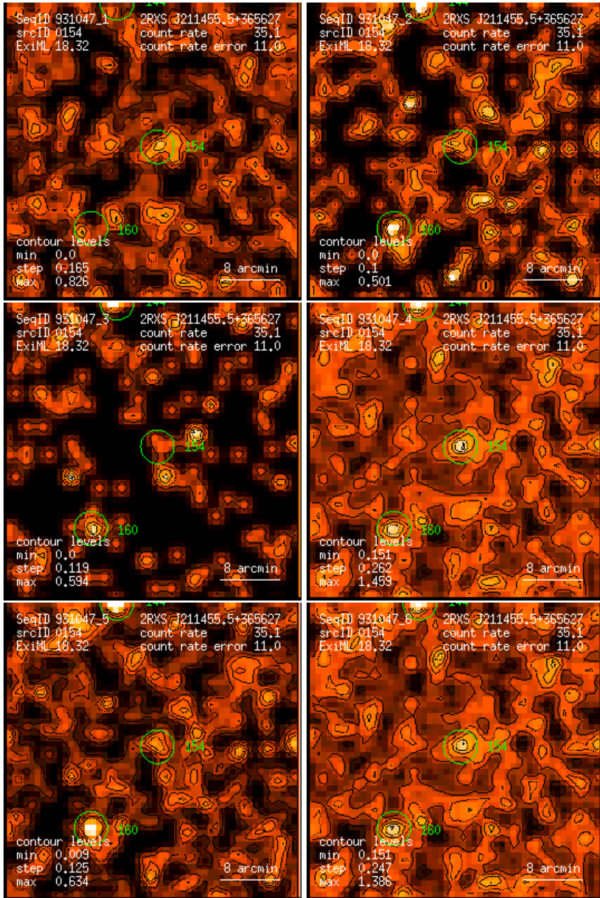
Figure 154: RASS 931047: detection 0154: band rate images, Gaussian filter: (1) PSPC channels 11 – 41, (2) 52 – 90, (3) 91 – 201, (4) 11 – 235, (5) 52 – 201, (6) 11 – 201. Broad band rates in counts/ks. Band rate contour levels in counts/ks/arcmin 2 .
