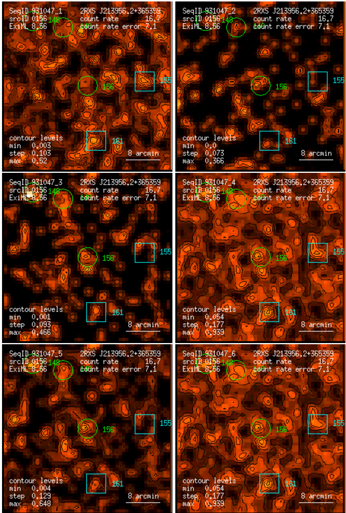
Figure 156: RASS 931047: detection 0156: band rate images, Gaussian filter: (1) PSPC channels 11 – 41, (2) 52 – 90, (3) 91 – 201, (4) 11 – 235, (5) 52 – 201, (6) 11 – 201. Broad band rates in counts/ks. Band rate contour levels in counts/ks/arcmin 2 .
