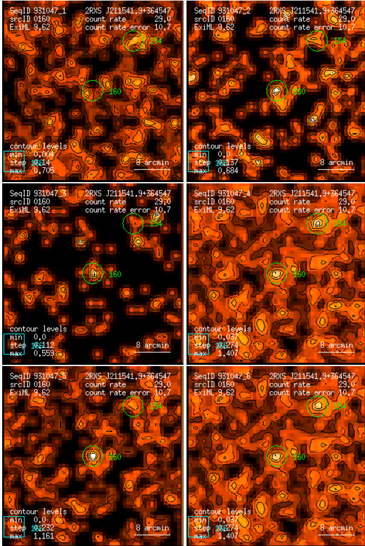
Figure 160: RASS 931047: detection 0160: band rate images, Gaussian filter: (1) PSPC channels 11 – 41, (2) 52 – 90, (3) 91 – 201, (4) 11 – 235, (5) 52 – 201, (6) 11 – 201. Broad band rates in counts/ks. Band rate contour levels in counts/ks/arcmin 2 .
