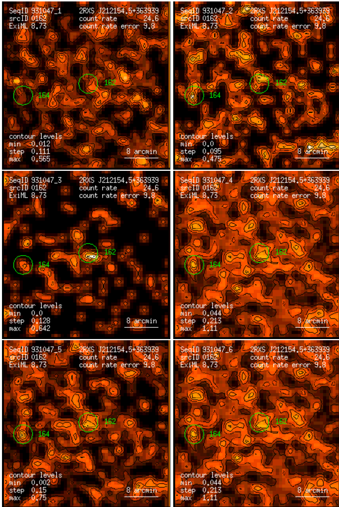
Figure 162: RASS 931047: detection 0162: band rate images, Gaussian filter: (1) PSPC channels 11 – 41, (2) 52 – 90, (3) 91 – 201, (4) 11 – 235, (5) 52 – 201, (6) 11 – 201. Broad band rates in counts/ks. Band rate contour levels in counts/ks/arcmin 2 .
