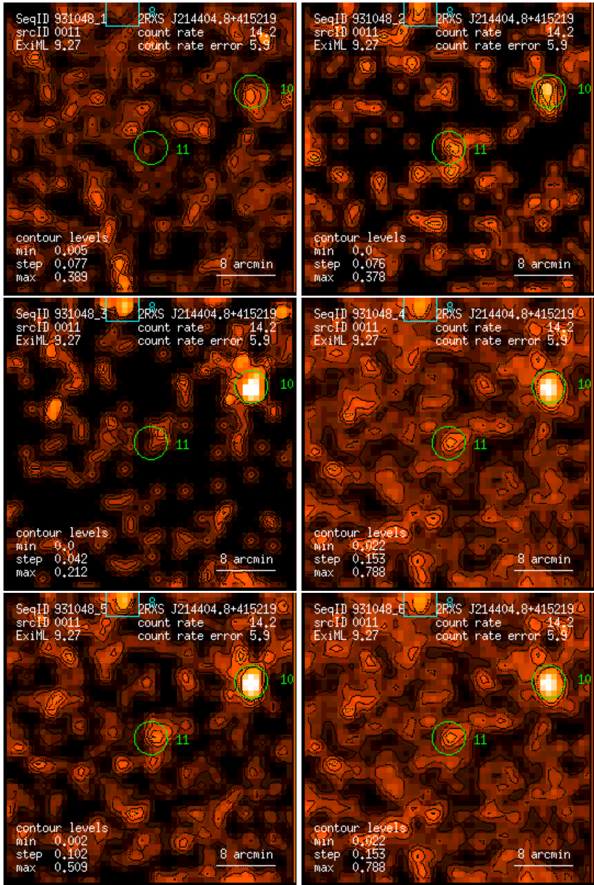
Figure 11: RASS 931048: detection 0011: band rate images, Gaussian filter: (1) PSPC channels 11 – 41, (2) 52 – 90, (3) 91 – 201, (4) 11 – 235, (5) 52 – 201, (6) 11 – 201. Broad band rates in counts/ks. Band rate contour levels in counts/ks/arcmin 2 .
